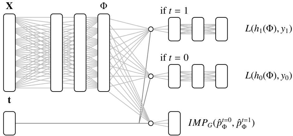
Figure 2.1: CFR architecture
