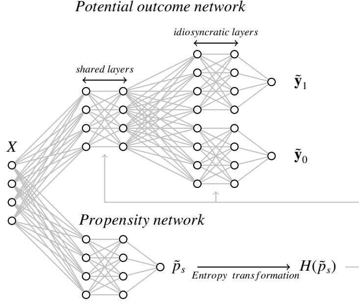
Figure 2.2: DCN-PD architecture
