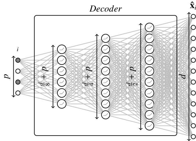
Figure 4.6: Decoder component of the Causal Auto-Encoder. It is composed of four layers for which the dimension is doubled at each layer. The dimension of the input is given by the size p fixed with the architecture of the latent space. The dimension of the output d is given by the dimension of covariates \mathbf{x}_i (number of features). The ReLU function is used as activation function at each layer.
