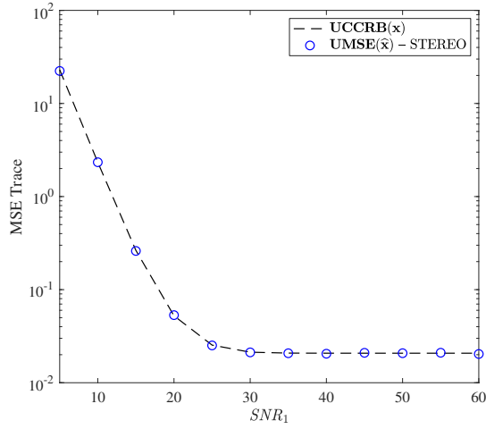
Figure 4.5: Scenario 1: UCCRB and UMSE from STEREO for \mathbf{x} , versus SNR_1 for fixed SNR_2 .
