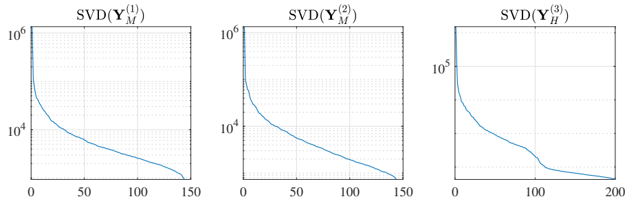
Figure 2.13: Singular values of the unfoldings, Indian Pines.
