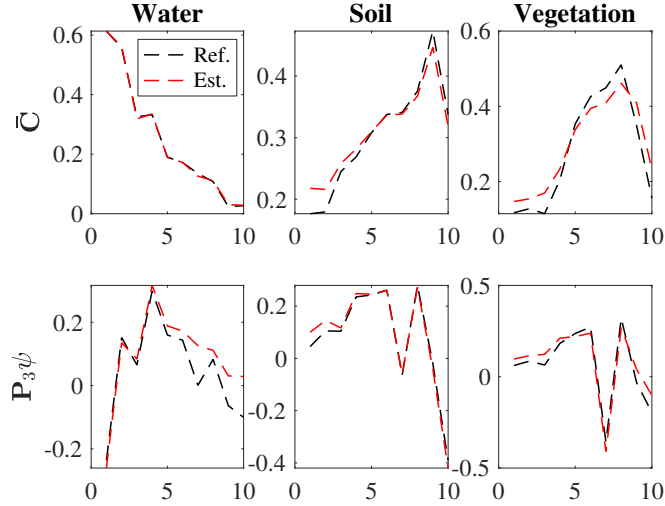
Figure 3.14: Reference and estimated \tilde{C}_M and \mathbf{P}_3\psi from CNN-BTD-Var, Lake Tahoe.
