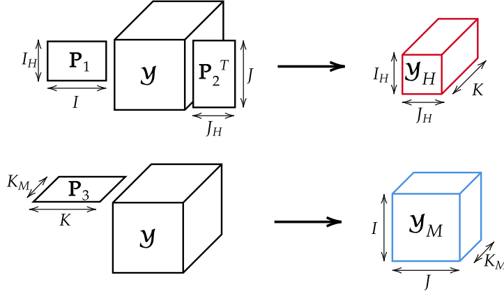
Figure 1.4: Noiseless tensor degradation model (1.28).
