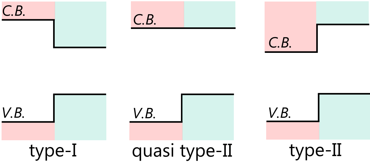
Fig. I.2 Diagram of the different possible band alignments in hetero-structure.
