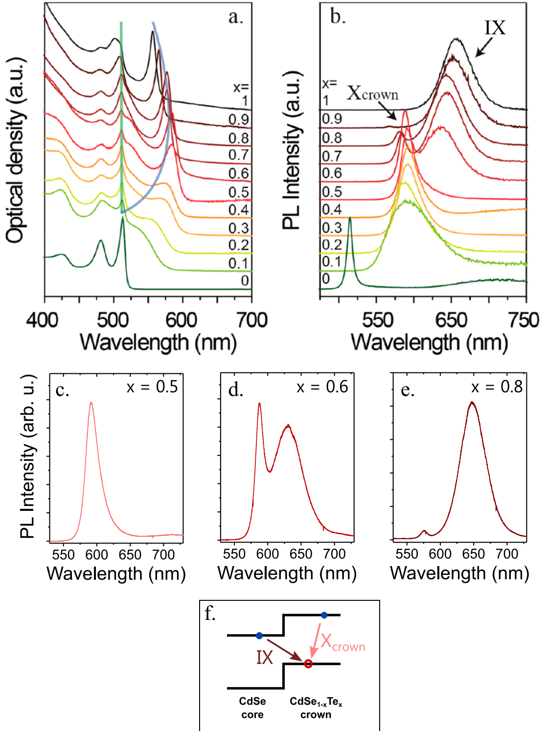
Fig. V.1 (a) Absorption of a solution of \text{CdSe}/\text{CdSe}_{1-x}\text{Te}_x NPLs at room temperature for x ranging from 0 to 1. The green line follows the signature of the heavy-hole transition in the \text{CdSe} core, while the grey bowed line follows the heavy-hole transition of the crown. (b) Its corresponding PL emission. For clarity the PL spectra of x = 0.5 (c), x = 0.6 (d) and x = 0.8 (e) are reproduced below. (f) diagram of the band alignment in \text{CdSe}/\text{CdSe}_{1-x}\text{Te}_x and the different recombination channels.
