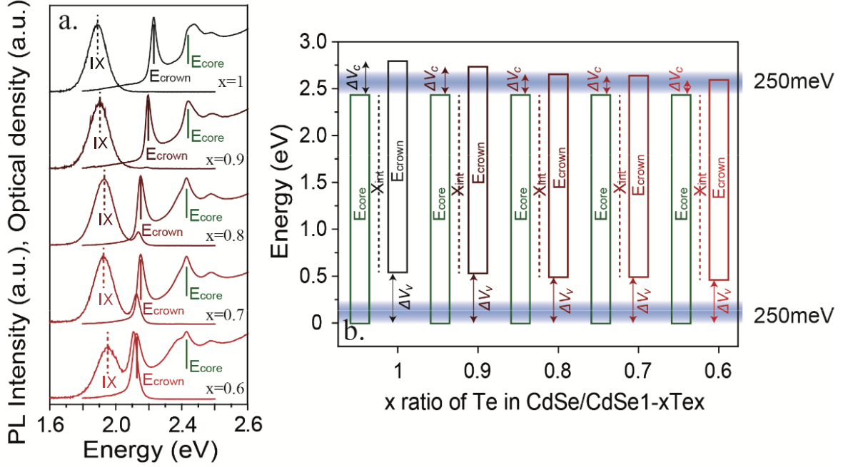
Fig. V.5 Determination of the band alignment of the CdSe core and the \text{CdSe}_{1-x}\text{CdTe}_x crown from the position of the absorption peaks of the core and the crown and the emission of IX. The 250 meV grey bands on the right diagram represent the binding energy of the direct X_{\text{crown}} exciton.
