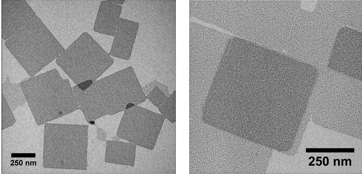
Fig. VI.5 TEM pictures of large square NPLs, obtained from the synthesis described in the text completed with the addition of 240 \mu\text{L} of HBr.
