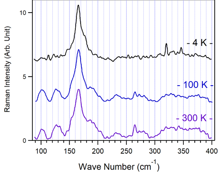
Fig. III.9 Raman spectra of a film of LC CdSe/CdTe NPLs at 4 K, 100 K and 300 K. A single peak at 166 \pm 2 \text{ cm}^{-1} ( = 20.6 \pm 0.3 \text{ meV} ) dominates the spectra at all temperatures. These measurements were performed by our collaborators in Cambridge.
