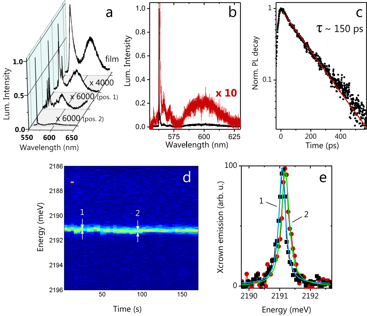
Fig. V.3 (a) PL spectra recorded for different dilutions of the initial \text{CdSe}/\text{CdSe}_{0.4}\text{CdTe}_{0.6} NPLs solution (b) PL spectrum of a single \text{CdSe}/\text{CdSe}_{0.4}\text{CdTe}_{0.6} NPL (black). The red trace represents the same spectrum multiplied by ten, to highlight the indirect exciton emission. (c) PL decay of the direct exciton X_{\text{crown}} from a single NPL and its mono-exponential fit with a time constant of 150 ps. (d) Trace of the X_{\text{crown}} emission over 170 s. (e) Spectra at the times marked 1 and 2 on the trace. A spectral shift of the emission is observed between the two times, while the shape is the same, characteristic of the spectral diffusion phenomena.
