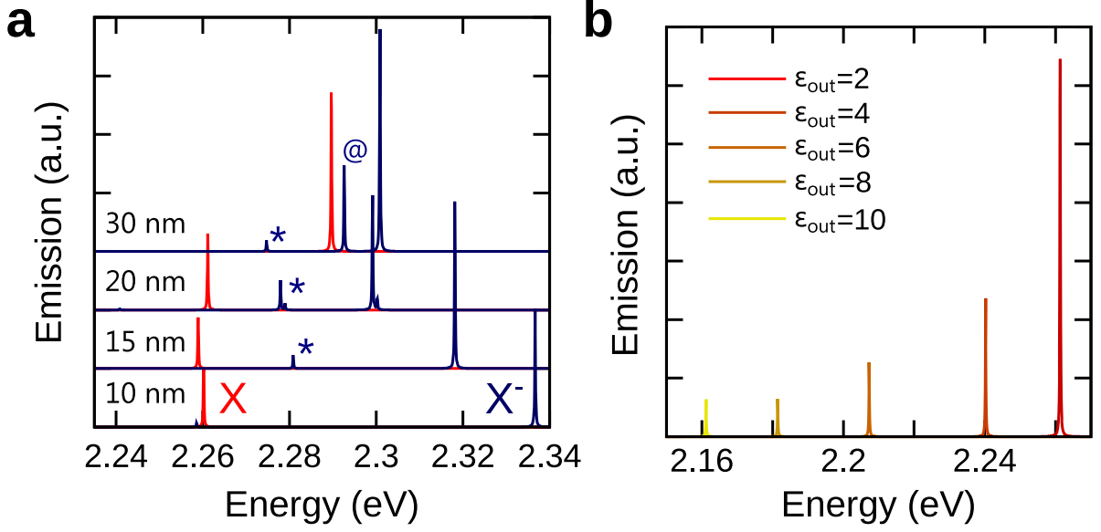
Fig. III.13 (a) Simulated emission spectra, at T = 7 K and \epsilon_{out} = 2 , of the neutral exciton ( X ) and negative trion ( X^- ) for L_y ranging between 10 nm to 30 nm. The lines labeled with an asterisk correspond to the so-called shake-up replicas and the one labeled with a @ corresponds to the recombination of a triplet trion. (b) Simulated emission spectra at T = 7 K of the neutral exciton with values of \epsilon_{out} ranging between 2 (dielectric constant of the organic ligands) and 10 (dielectric constant of CdSe and CdTe).
