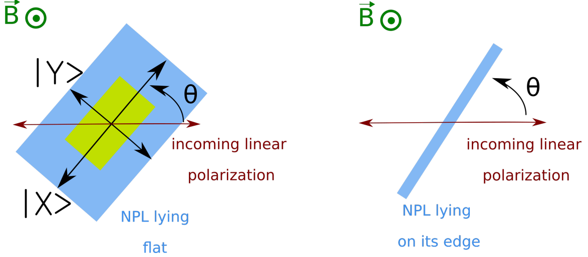
Fig. IV.9 Sketch of the orientation of the NPLs compared to the incoming polarization.
