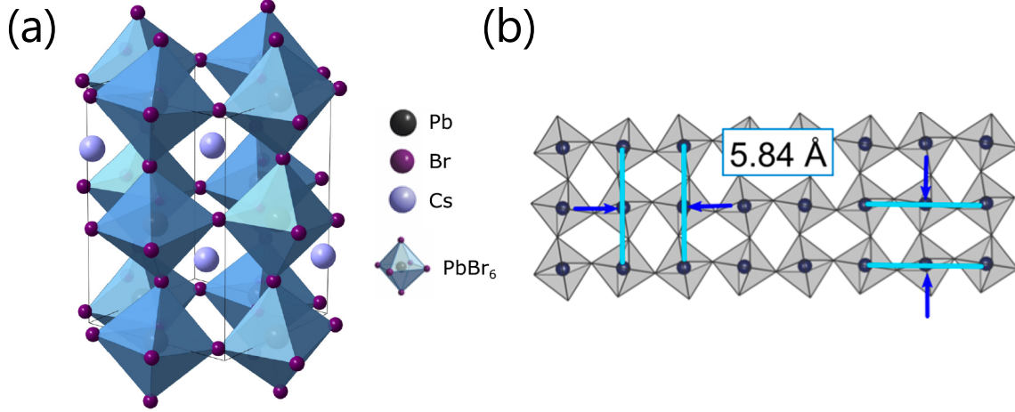
Fig. VI.1 (a) Sketch of the orthorhombic perovskite unit cell (adapted from ref. [33]). (b) Diagram of the facets of \text{CsPbBr}_3 NPLs, highlighting the inter-planar distance, a = 0.58 \text{ nm} (adapted from ref. [36]).
