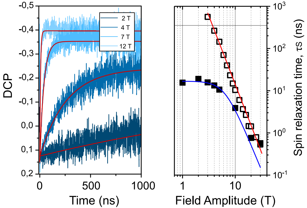
Fig. IV.4 On the left side: DCP(t) for different value of the B -field and their mono-exponential fit (red). On the right side: evolution of \tau_s , the spin relaxation lifetime for T = 1.6 K (open squares) and T = 25 K (filled squares). The red and blue lines are the adjustment of these curves with aB^{-3.2} and 1/(\Gamma_{S,0} + kB^{-3}) with 1/\Gamma_{S,0} = 17 ns, respectively. The grey horizontal line corresponds to the relaxation lifetime, \tau_r = 350 ns, at 1.6 K, obtained from the average of the different multi-exponential components (see IV.1.2.b).
