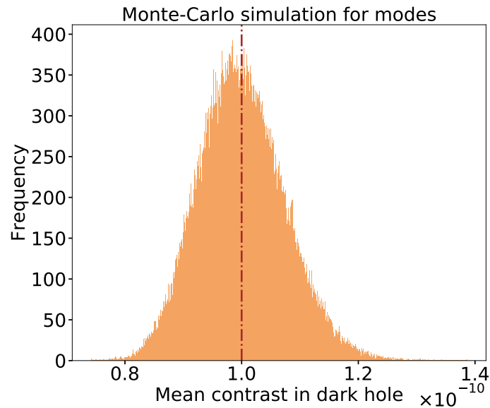
Figure 2.12: Validation of the uniform contrast allocation across PASTIS modes with an E2E Monte-Carlo simulation, drawing random sets of mode weights from a normal distribution with standard deviations \sigma (Eq. 2.28), corresponding to an equal contrast allocation per mode (Eq. 2.26) with weights \tilde{\mathbf{b}} . The overall WFE of one realization is the sum of all weighted modes for each set, and is propagated in an E2E simulation. The histogram represents 100,000 realizations of the average dark hole contrast for a target contrast of 10^{-10} .
