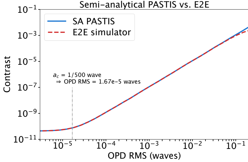
Figure 2.4: Average dark hole contrast as a function of wavefront error using both an end-to-end simulator (dashed red) and the PASTIS matrix propagation (solid blue). In a hockey stick graph behavior, the contrast is limited by the coronagraph itself at low wavefront errors corresponding to the flattened out curve to the left (at c_0 ). From about 10^{-4} waves to 10^{-1} waves of WFE RMS, the contrast is limited by segment phasing aberrations. In this range the estimation error of PASTIS is 0.06% compared to the reference E2E model. A calibration aberration per segment a_c of 1/500 wave, on a 120 segment pupil, translates to a global WFE of 1.67 \times 10^{-5} waves when calibrating the PASTIS matrix diagonal, or 2.36 \times 10^{-5} with two simultaneously aberrated segments, which is in the small aberration regime of the model, just above the coronagraph floor. The curves shown are obtained as the mean of the same 20 random realizations for each RMS value, both for the E2E simulator and the PASTIS propagation. At large wavefront errors (close to 0.1 waves RMS) the linear approximation breaks down and the two curves no longer match perfectly.
