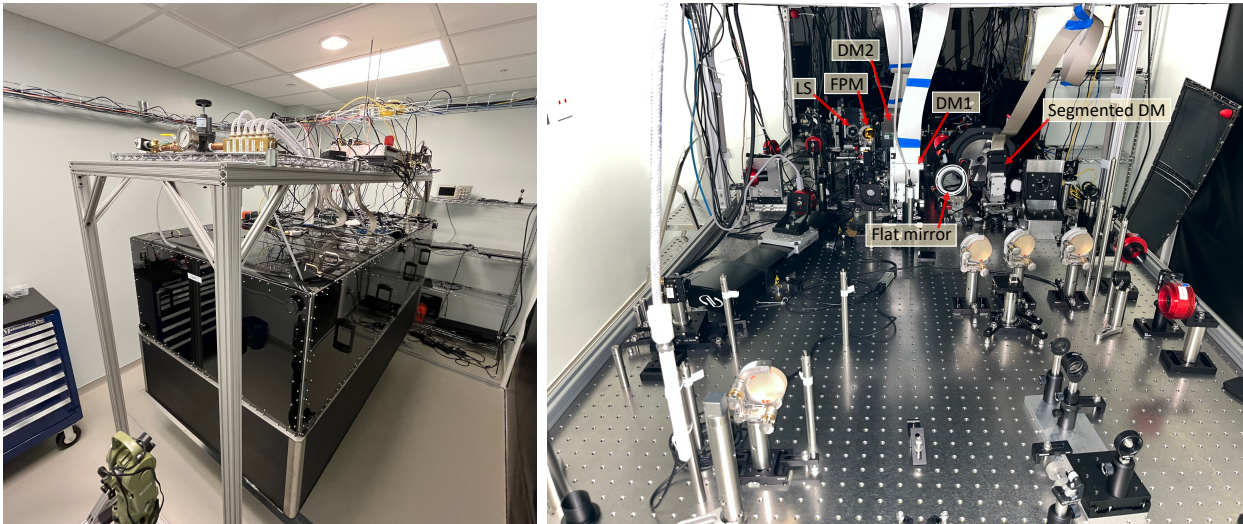
Figure B.1: Left: HiCAT enclosure in its cleanroom, mounted on a floating optical table. The theodolite in the bottom left is used for fine alignments during component changes. Right: Frontal view of the HiCAT testbed with unmounted enclosure panels. The light source injection unit is located in the far right corner and is not visible in this image. The white wide cables belong to the three DMs installed on the testbed (the two Boston continuous DMs to the left and the IrisAO segmented DM to the right; DM1 and the segmented DM are seen from the back). The red cylindrical pieces are various CMOS camera models by ZWO that are used both as science and pupil cameras, as well as the detector for the Zernike wavefront sensor and as alignment cameras in the Michelson interferometers. The testbed mode in this image is a “segmented CLC” mode where the apodizer is replaced by a high-quality flat mirror.
