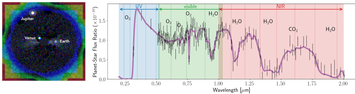
Figure 1.7: Our goal: observe an exoEarth with confirmed biomarkers. Left: Simulated image of a solar system analogue at a distance of 12.5 pc as seen with the 15 m diameter LUVOIR A space telescope, using an apodized pupil Lyot coronagraph (APLC). After a realistic application of starlight suppression with a coronagraph, WFE influence, noise and post-processing, the planets become clearly visible, among them an Earth-twin. Right: Simulated spectrum of an exoEarth with ECLIPS, the coronagraphic imaging instrument on LUVOIR, modeled after the Earth as we know it today. Data like these will allow us to measure abundances of molecules in the atmospheres of planets, with the goal to identify habitable conditions. Shaded regions mark 20% bandpasses in the near-UV (blue) and optical (green), and 10% bandpasses in the near-IR, with the vertical lines in the bandpass centers. Source: The LUVOIR Team (2019).
