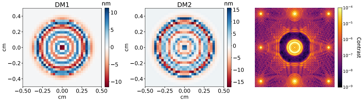
Figure 2.19: Final DM surface commands for a baseline contrast c_0 = 6 \times 10^{-8} obtained with iterative pair-wise estimation and stroke minimization on a non-segmented CLC simulation of the HiCAT testbed without any WFE. The DM surfaces are the main contributor to the phase term \phi_{DH} in Eq. 2.43, describing the elements of the PASTIS matrix. The pair-aberrations are applied on top of these surface commands when the PASTIS matrix is built and the resulting average contrast is measured in the circular DH with an extent of 6\text{--}11 \lambda/D_{LS} .
