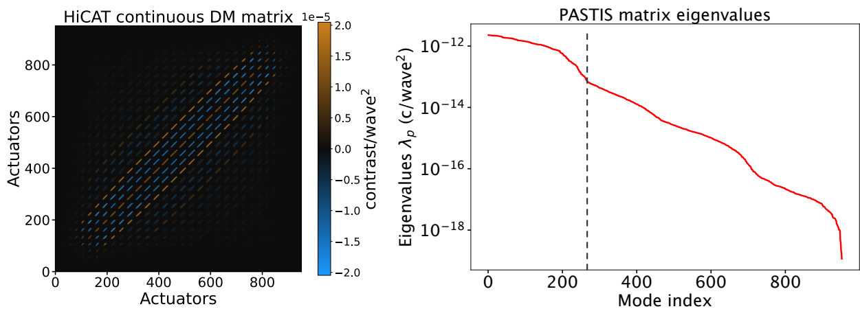
Figure 2.20: HiCAT PASTIS matrix (left) and eigenvalues (right) for the pupil-plane continuous DM with 952 individual actuators. Left: The chopped-up structure in the matrix is a result of the actuator numbering on the DM: instead of going outwards in spirals starting from the center, the actuators are numbered row by row. Since the actuators at either end of each row are not illuminated, their influence on contrast is negligible. Right: The eigenvalues span almost seven orders of magnitude and suggest that there are at least three different eigenmode regimes with different relevance for the contrast. The dashed vertical line marks the point where noise starts dominating the eigenmodes.
