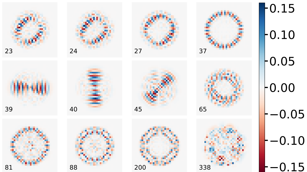
Figure 2.21: Pupil-plane eigenmodes for the continuous PASTIS analysis on HiCAT, with their respective mode index corresponding to the eigenvalues in Fig. 2.20, right. Modes with an index up to \sim 270 , marked by the vertical dashed line in Fig. 2.20, have a significant impact on the coronagraph contrast, as quantified by the respective eigenvalue.
