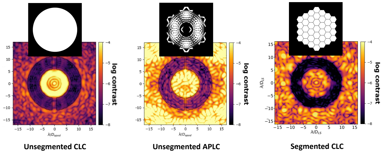
Figure B.3: Three of the different testbed modes in which HiCAT can be operated. The experimental DH results in the unsegmented modes (left and center) were obtained without the IrisAO segmented DM installed in the beam, the segmented mode (right) does include the segmented DM. All the DHs were obtained with a WFS&C loop using PW and stroke minimization. We note how the angular scale in the left two images is indicated in units of \lambda/D_{apod} , while the right DH is shown in units of \lambda/D_{LS} . At the time of writing, the best monochromatic contrast on HiCAT has been achieved in the segmented CLC mode (right), with an average contrast of 2 \times 10^{-8} in a DH from 6 - 10\lambda/D_{LS} . Not shown is the anticipated “full” testbed mode of HiCAT, the segmented APLC.
