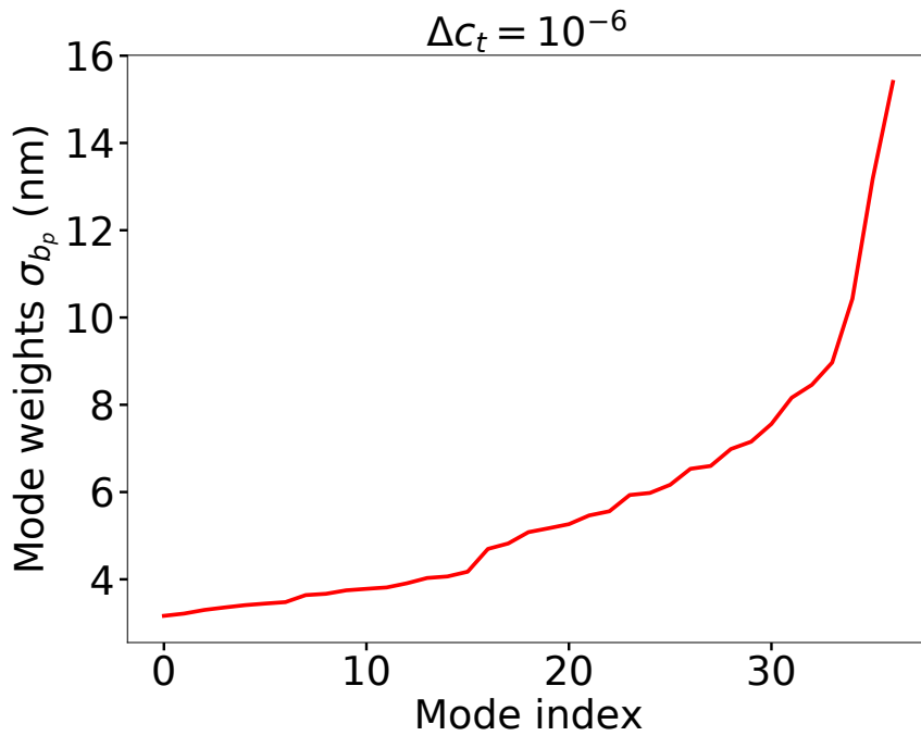
Figure 4.9: Mode requirements as calculated with Eq. 4.17 for a uniform contrast contribution per mode to a differential target contrast of 10^{-6} . These are used as modal weights in the cumulative contrast measurement shown in Fig. 4.10.
