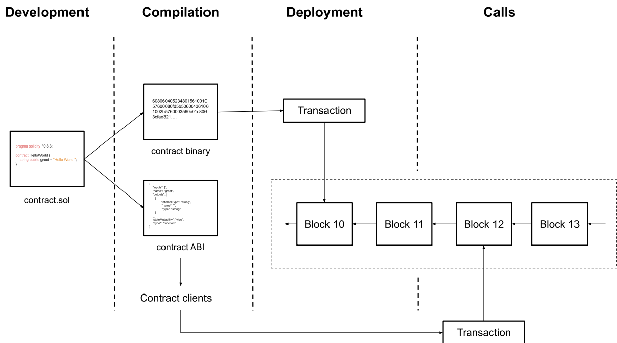
Figure 2.11 – An Ethereum contract's lifecycle
