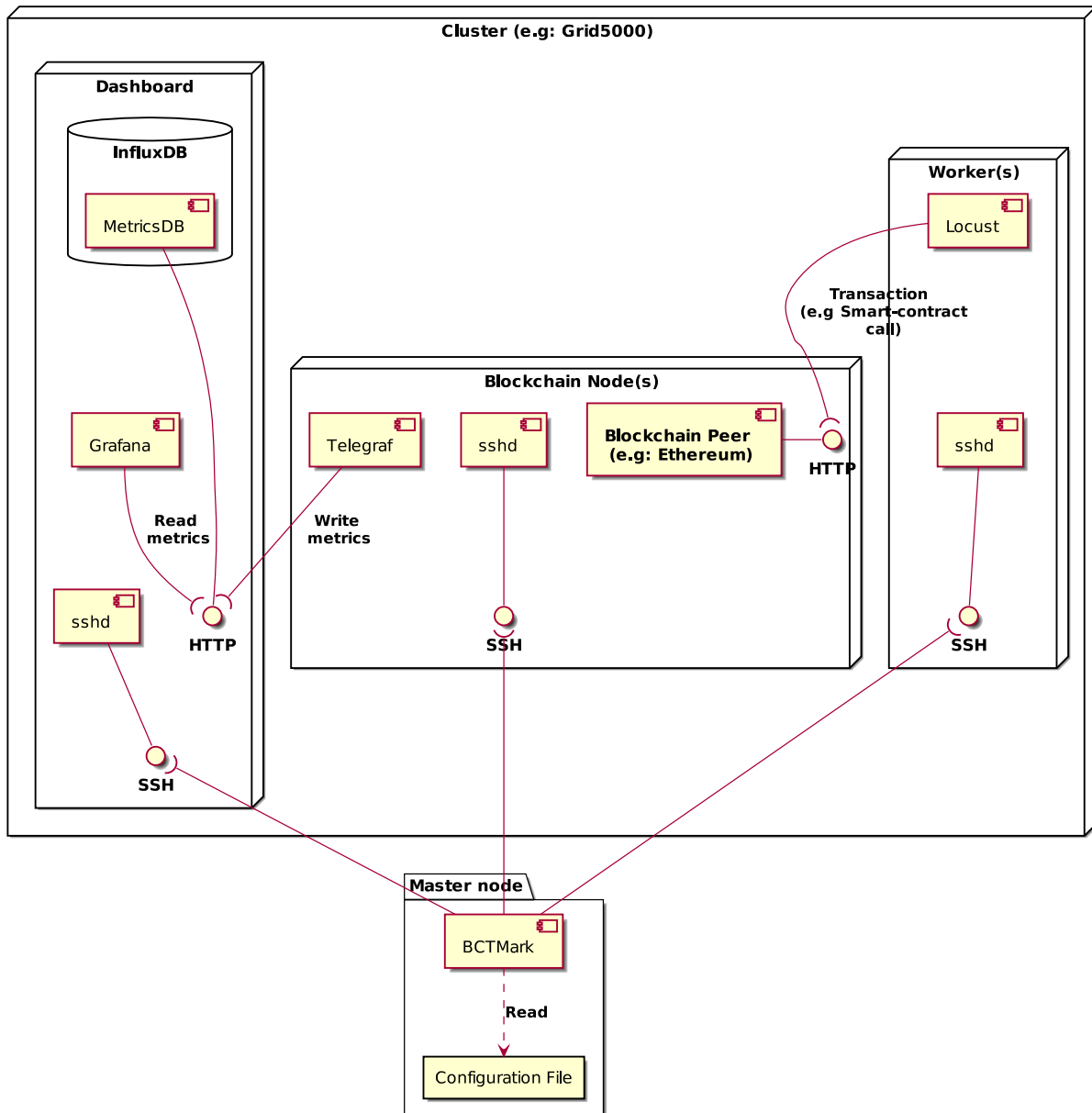
Figure 4.2 – BCTMark architecture
