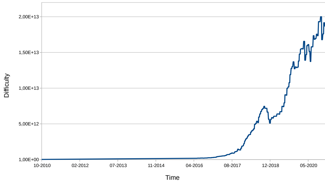
Figure 3.1 – Evolution of Bitcoin difficulty through time (data source: https://www.blockchain.com )
