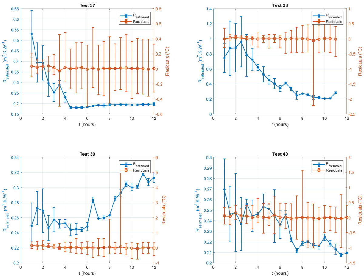
Figure A4.6: Estimated thermal resistance and residuals between measured and estimated minimization parameter for the four tests on the SW wall under variable conditions with the third prototype.
