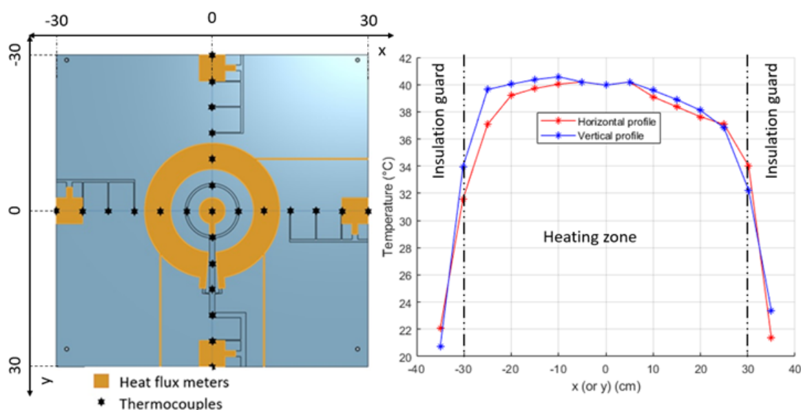
Figure 4.20: Horizontal and vertical profiles of wall surface temperature measured by thermocouples on the aluminum plate during measurement.
