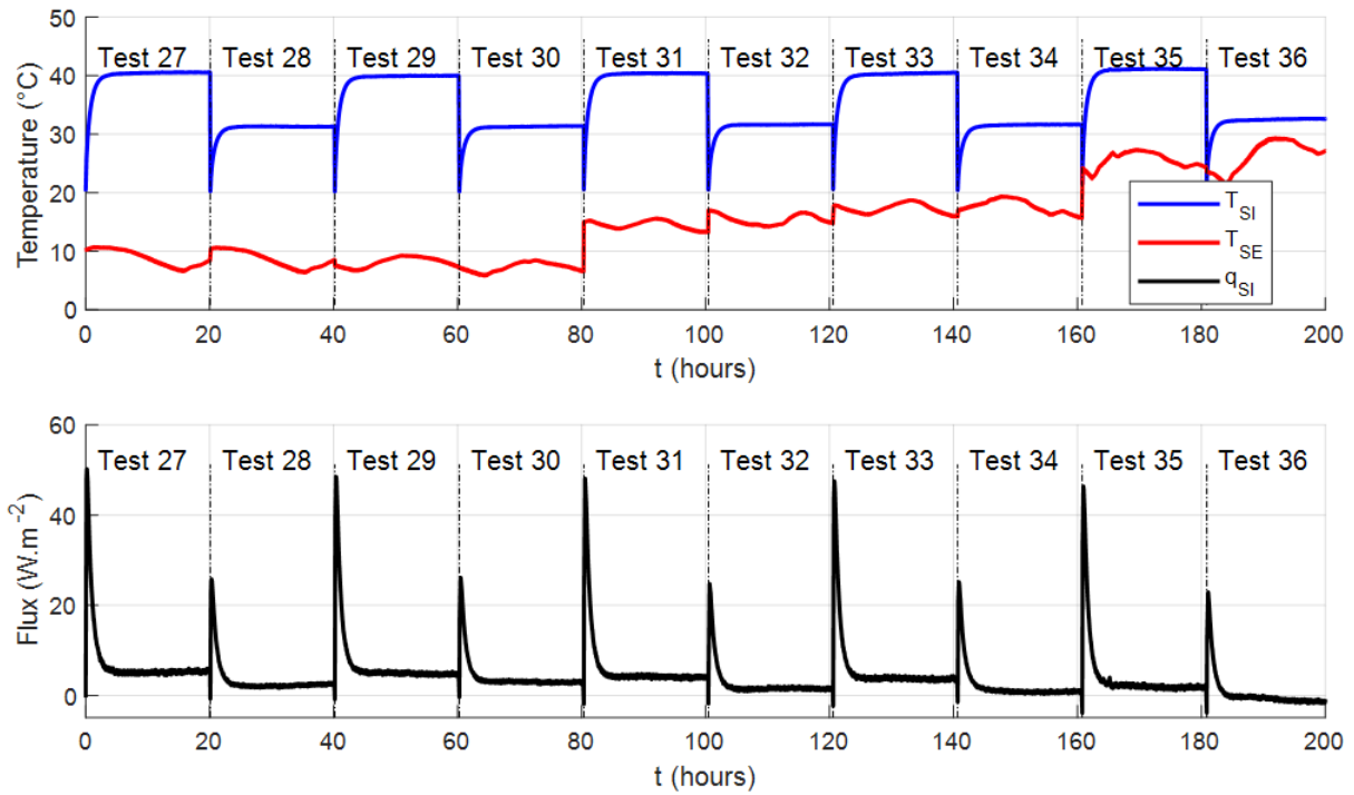
Figure 6.13: Measurement data for the IWI tests 27 to 36 with the third prototype under variable environmental conditions.
