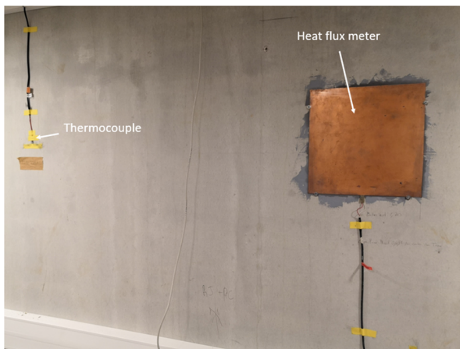
Figure 5.9: Thermal sensors on the internal surface of the tested SW wall used to apply the Heat Flux Meter method.
