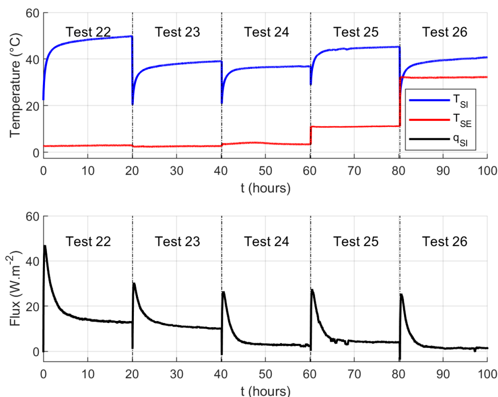
Figure 6.10: Measurement data for the WFW tests 22 to 26 under constant environmental conditions.
