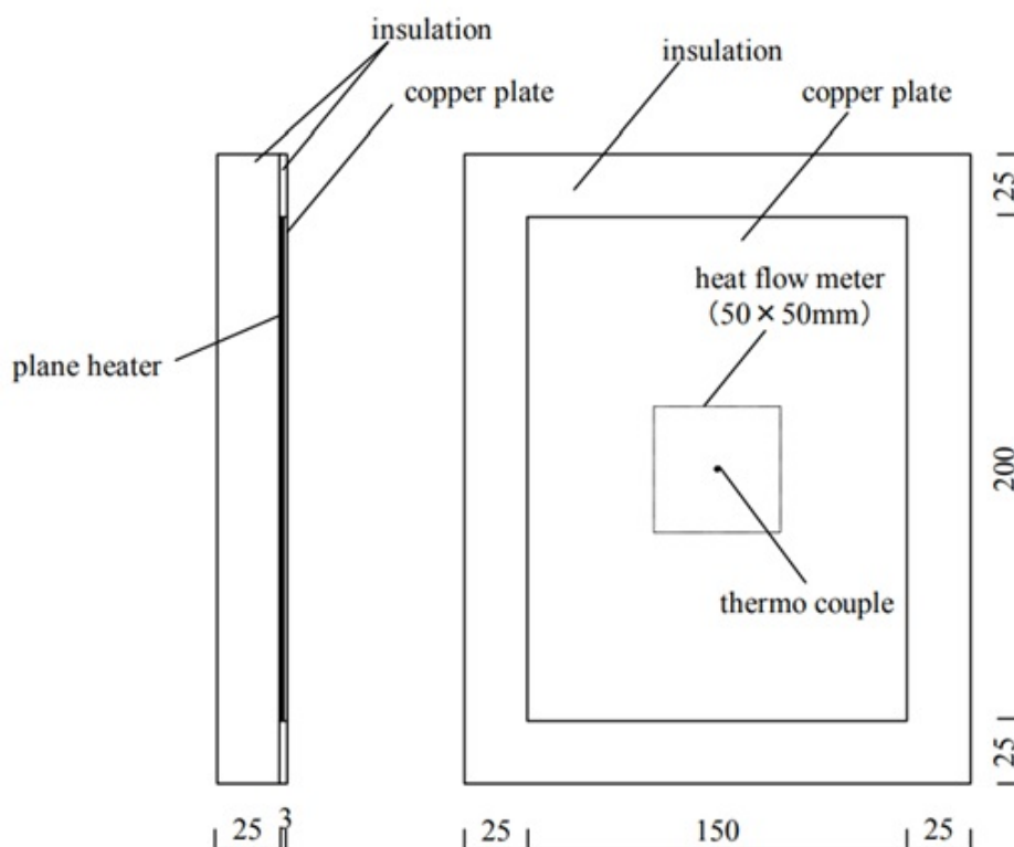
Figure 1.9: Outline of first additional element in [25].
