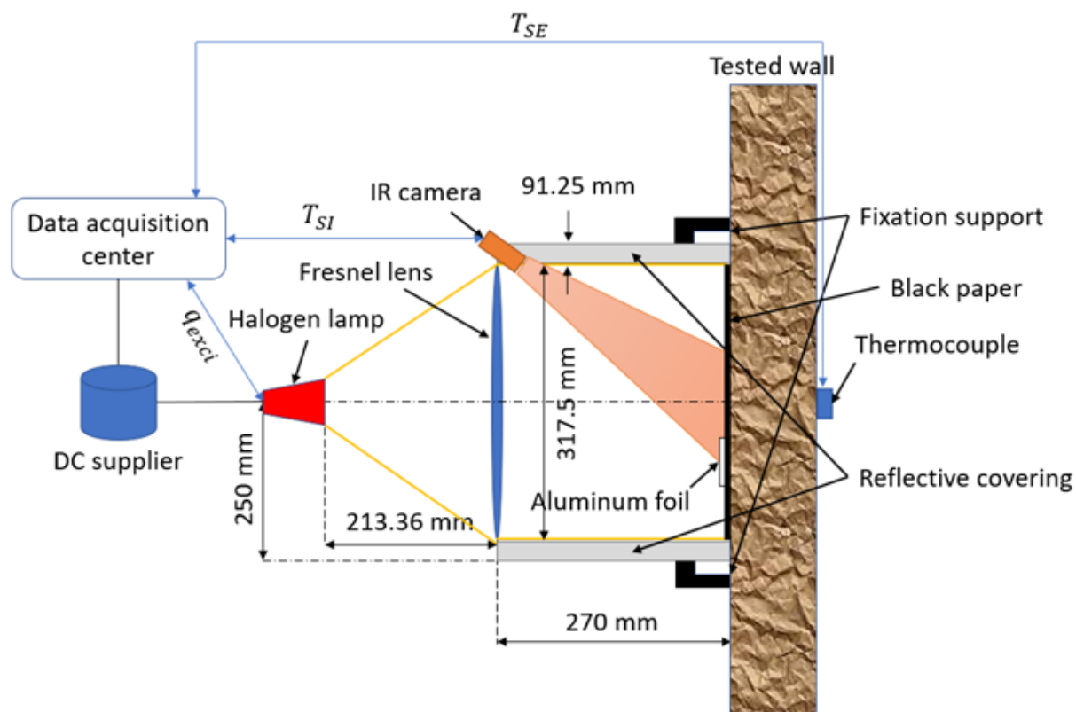
Figure 4.5: Schematic view of the first prototype.
