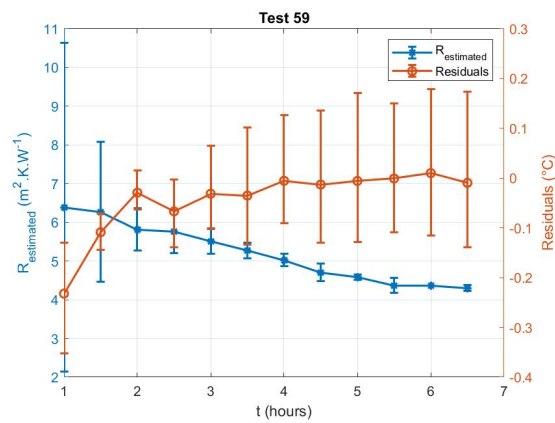
Figure A4.10: Estimated thermal resistance and residuals between measured and estimated minimization parameter for the nine tests on the IWI wall under variable conditions with the fourth prototype.
