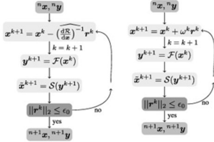
Figure 3.31: Simplified scheme of (Left) the IQN-ILS technique, and (Right) Aitken relaxation (adapted from (Degroote et al., 2009))
