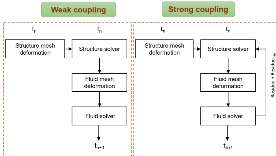
Figure 3.30: Solving process for a fluid-structure interaction problem with weak coupling and strong coupling using the partitioned approach.
