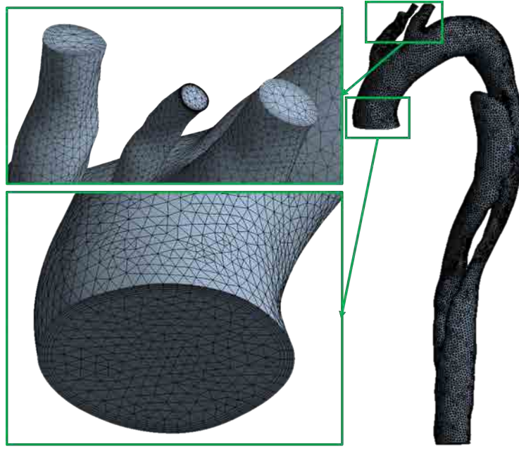
Figure 3.7: Tetrahedral mesh generated with the commercial software ANSYS® (1575416 cells)
