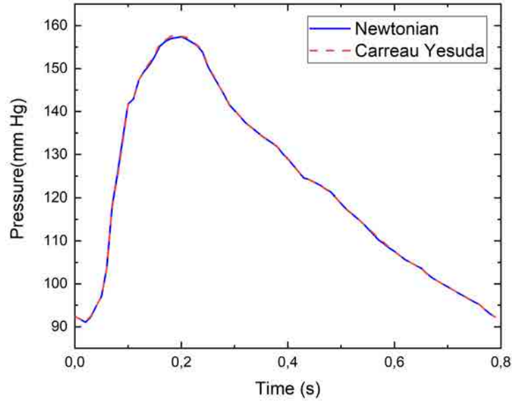
Figure 3.23: Pressure on section C (TL & FL section) for the Newtonian and Carreau-Yasuda models with a cardiac cycle
