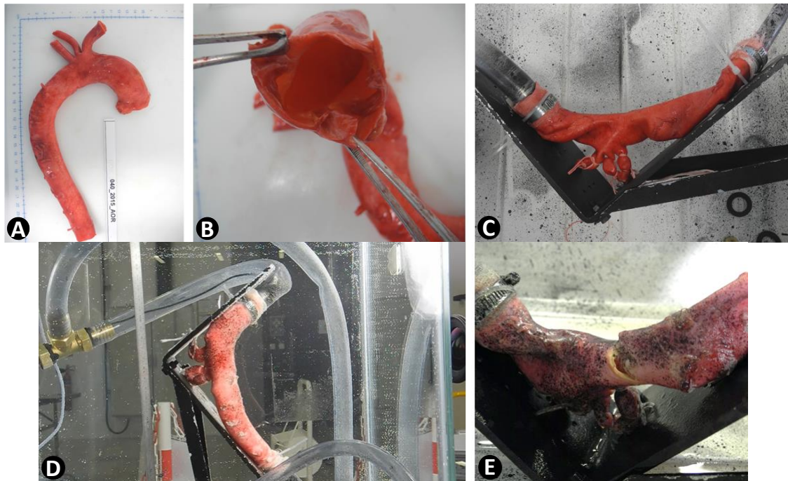
Figure 2.24: (A) Sample cleaned (B) The inside of the thoracic arch reveals no signs of calcification for this fresh sample (C) Installation of the speckled sample on its support (D) Aorta immersed in water before the experiment (E) Rupture on the aortic isthmus ( Menut et al., 2015 )
