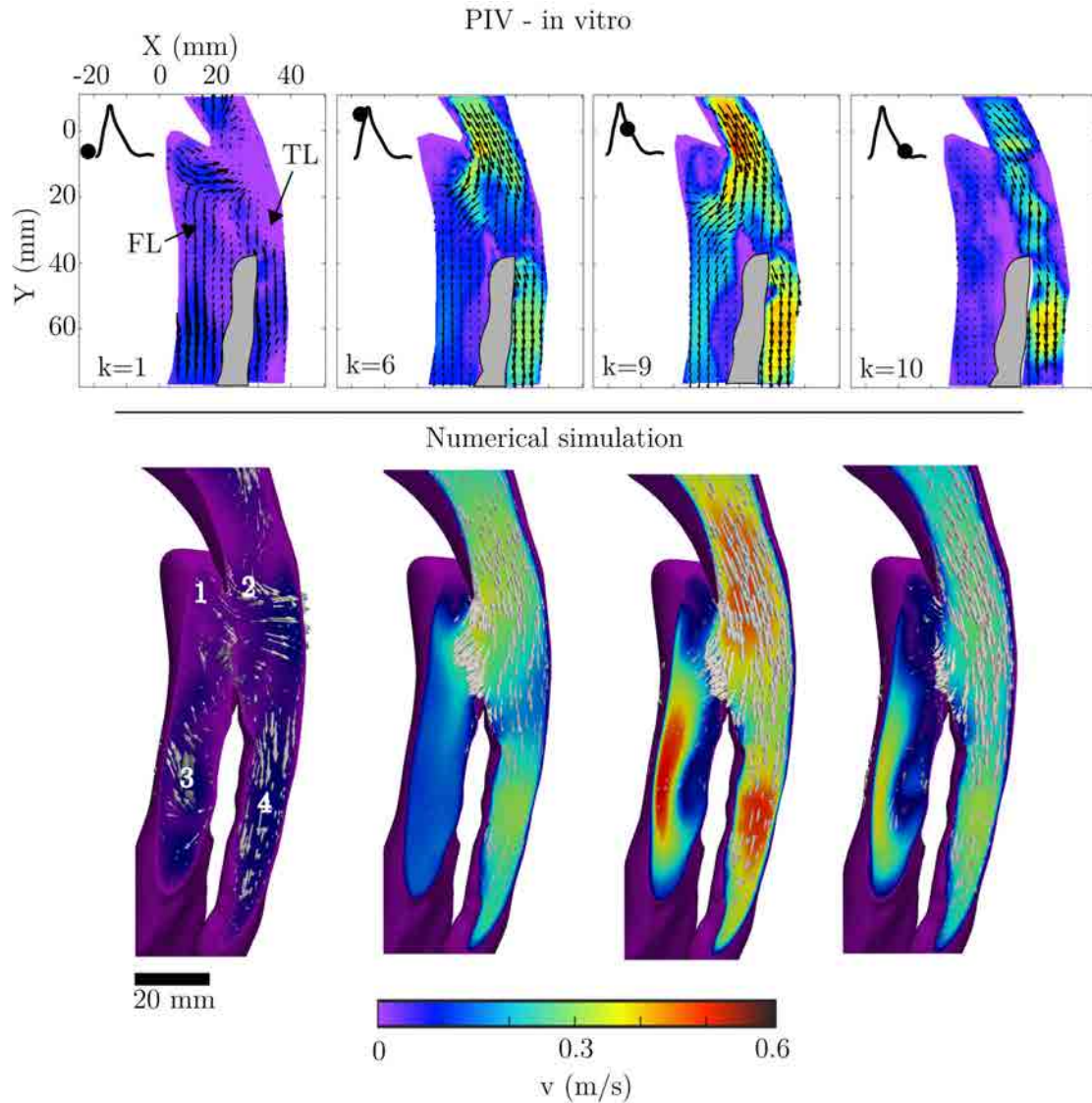
Figure 4.30: Comparison of PIV and numerical simulation velocity results for AD1 at four instants
