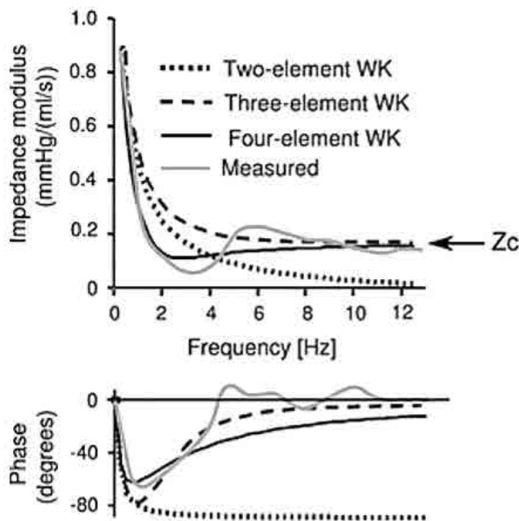
Figure 3.14: An example of measured impedance at the aortic inlet and impedances predicted by the two-element, three-element and four-element Windkessel model ( Westerhof et al., 2009 )
