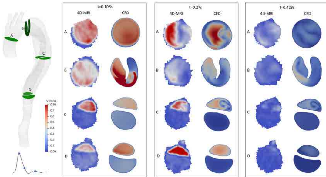
Figure 4.11: Velocity profiles on several sections along the aorta and compared with 4D-MRI
