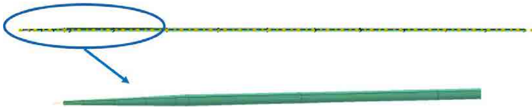
Figure 3.43: Modeling of the catheter (stent holder) whose elastic mechanical properties are derived from results of Mouktadiri (2013)
