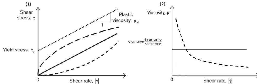
Figure 2.3: (1) Shear stress versus shear rate diagram for Newtonian (solid line) and non-Newtonian fluids in a simple shear flow. The dotted line represents a non-Newtonian fluid with a yield stress. The top dashed line indicates shear-thinning fluid without yield stress. The bottom dashed line represents shear-thickening fluid without yield stress. (Bao et al., 2017) (2) Viscosity-shear rate relationships for Newtonian (solid line) and non-Newtonian (dashed line) fluids
