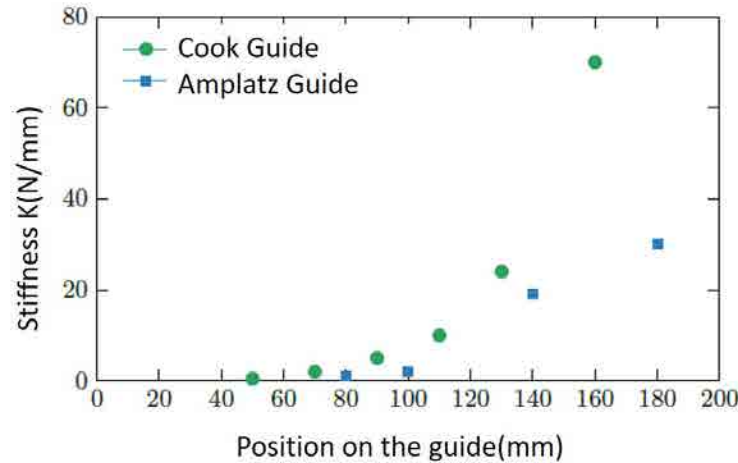
Figure 2.31: Evolution of stiffness along the transition zone of the Cook and Amplatz guides (Menut, 2017)
