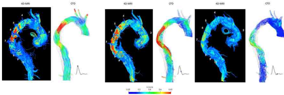
Figure 4.16: Flow streamline comparison between 4D-MRI data and postoperative CFD model
