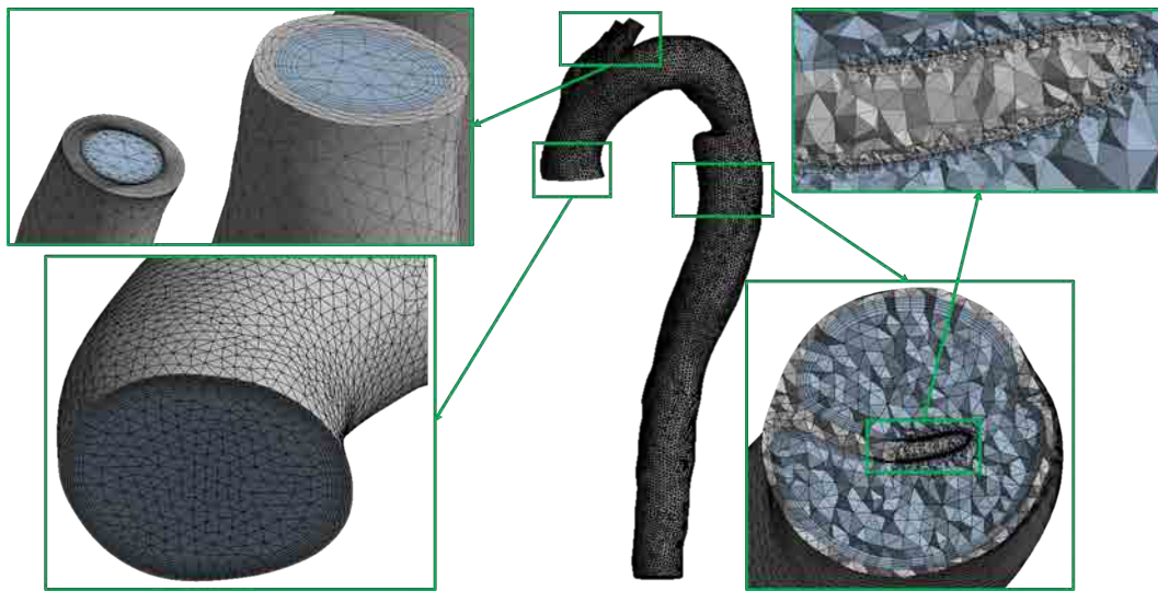
Figure 3.32: tetrahedral mesh generated with the commercial software ANSYS©
