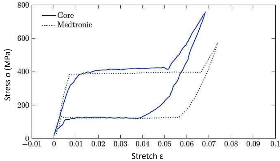
Figure 2.28: Comparison of cyclic tensile test curves (1 cycle represented) for Gore and Medtronic Nitinol stents (Menut, 2017)
