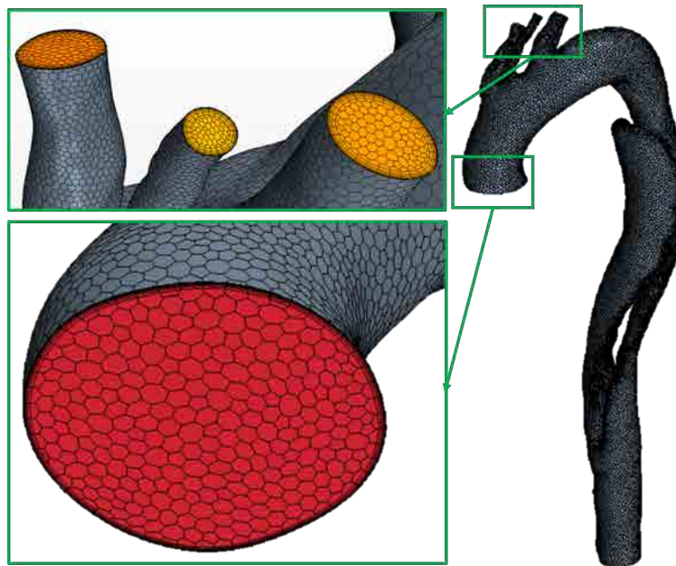
Figure 3.6: Polyhedral mesh generated with the commercial software Star-CCM+ © (338265 cells)
