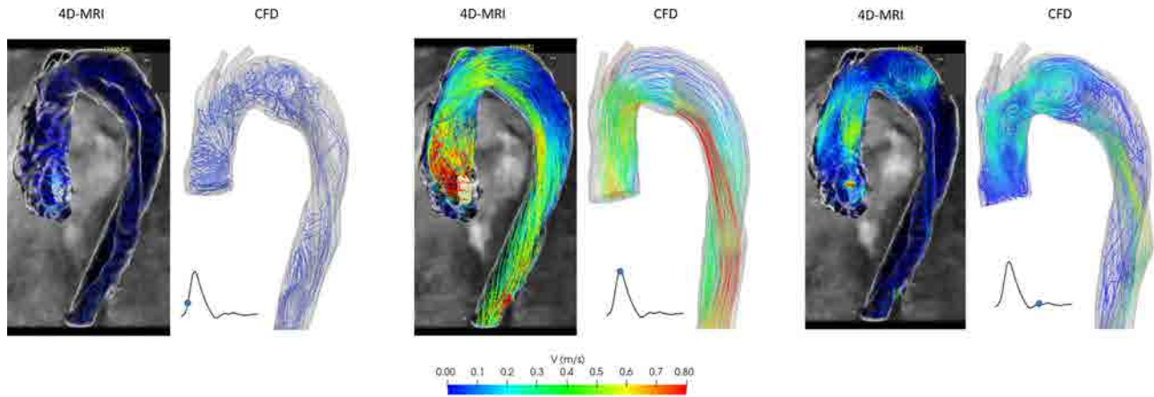
Figure 4.13: Comparison the flow streamline between 4D-MRI data and CFD simulation of preoperative
