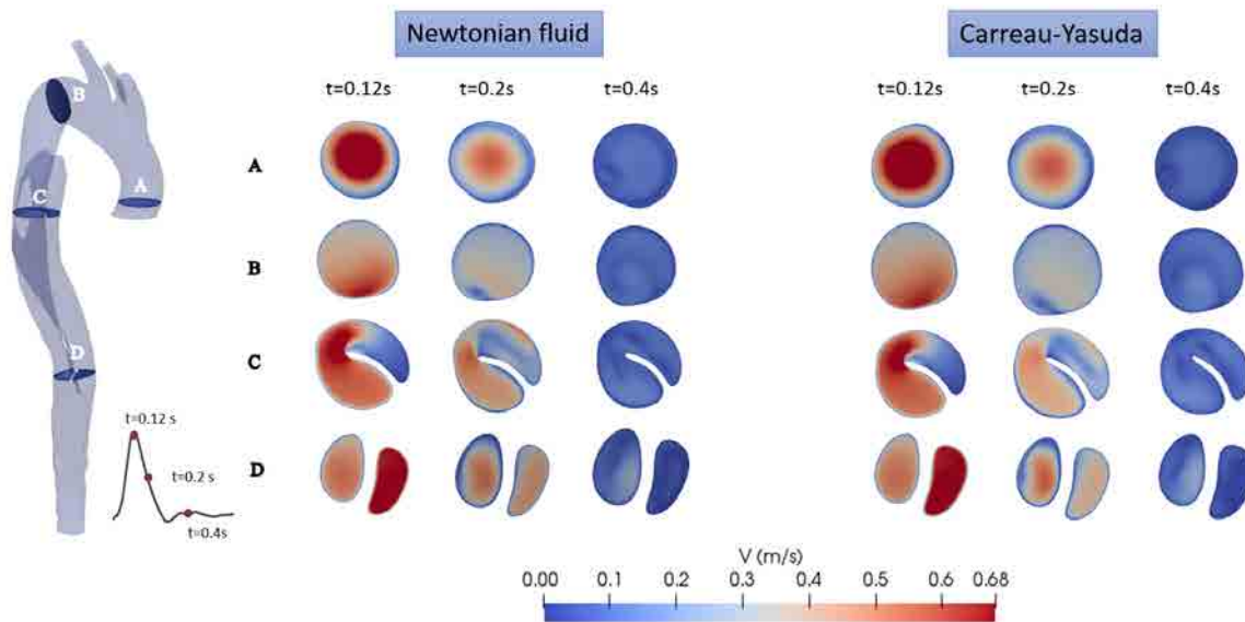
Figure 3.20: Velocity profiles on several sections along the aorta for the Newtonian and Carreau-Yasuda models
