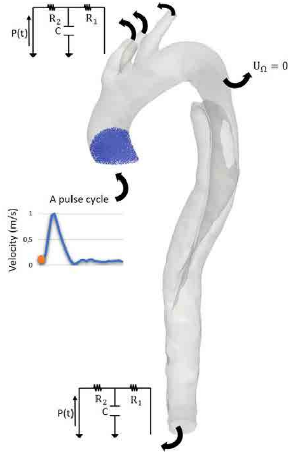
Figure 3.16: Diagram of the configuration of the numerical model with rigid walls on OpenFOAM
