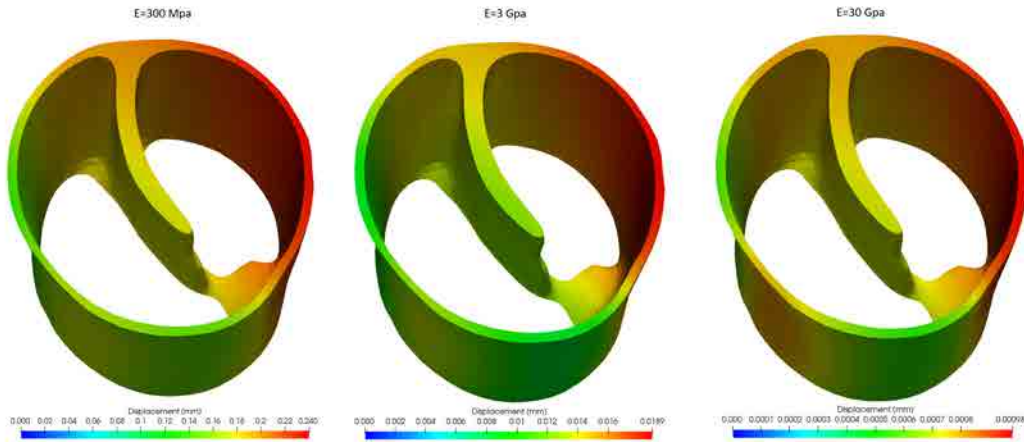
Figure 3.39: Displacement of IF region with various Young's modulus at peak systole
