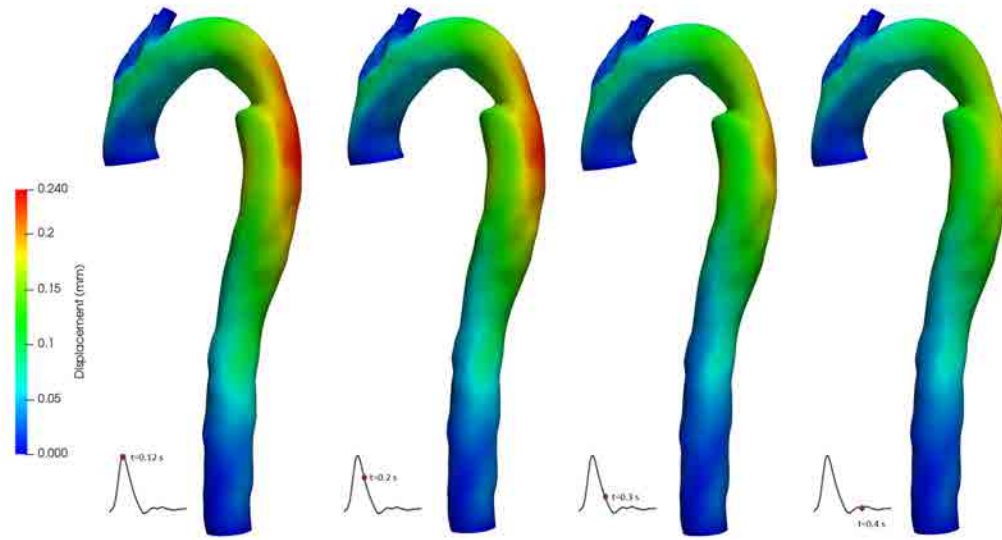
Figure 3.37: Displacement of the artery at various time instances with Young's modulus = 300 MPa
