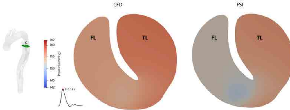
Figure 3.35: Comparison of the pressure at peak systole between CFD and FSI models on the place of Section C
