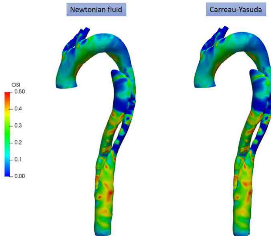
Figure 3.27: Comparison of OSI between the Newtonian and Carreau-Yasuda models
