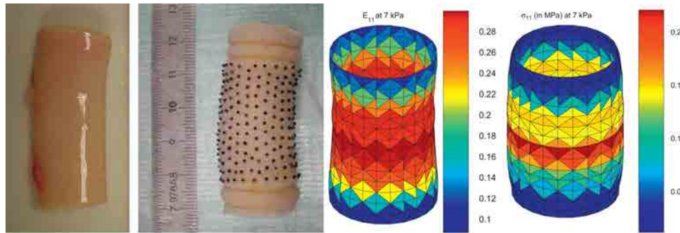
Figure 2.21: (Left) Image of the thoracic aorta section used for testing (Middle) Green-Lagrange strains in the initial configuration (Right) Cauchy tensor stresses in the deformed configuration (Avril et al., 2010).
