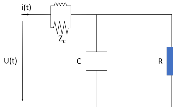
Figure 3.13: The four-element Windkessel model introduces an inductance L modeling the low-frequency blood inertia in parallel with the impedance Z_C connected in series with the two-element Windkessel model.
