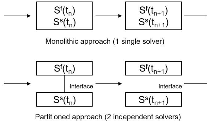
Figure 3.29: Schematic of monolithic and partitioned approaches for FSI
