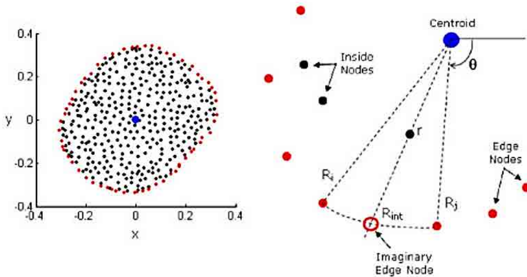
Figure A.1: A diagram illustrating how to transfer a radial velocity profile onto the nodes of a 2D boundary surface ( Mynard and Nithiarasu, 2008 )
