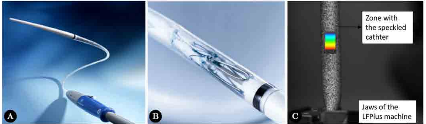
Figure 2.32: (A-B) Catheter with an undeployed stent inside (images from Medtronic©) (C) Traction testing of the stent-containing portion speckled in white on a black background (Mouktadiri, 2013)
