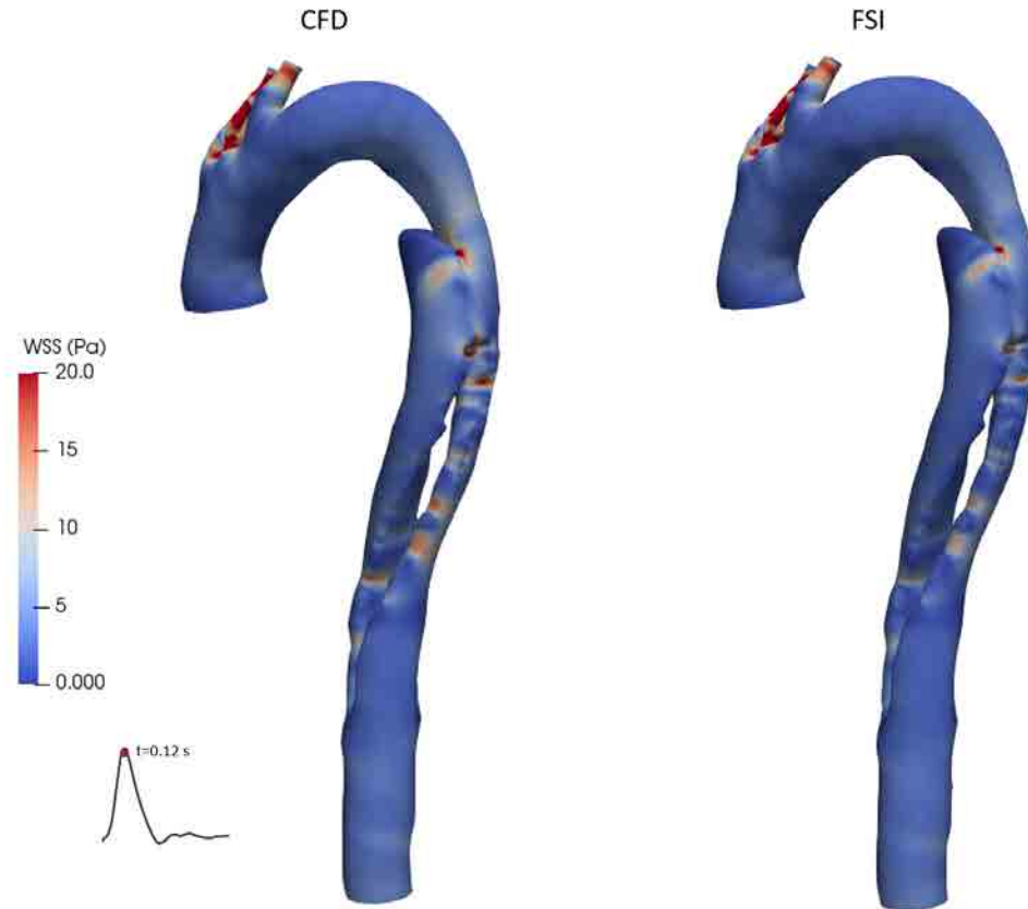
Figure 3.36: Comparison of the WSS at peak systole between CFD and FSI models
