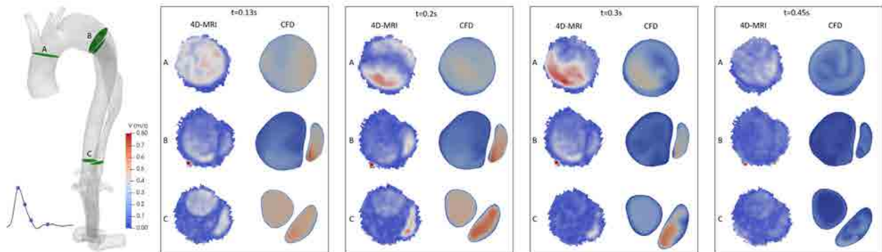
Figure 4.14: Velocity profiles on several sections along the aorta and compared with 4D-MRI
