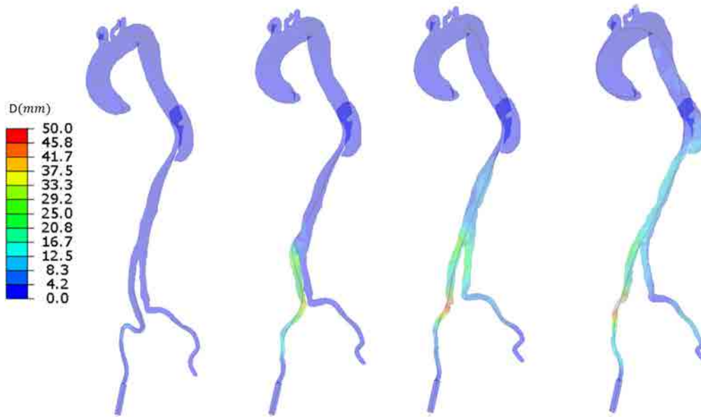
Figure 3.47: Displacement of aorta observed on the Amplatz guide during rise in the thoracic aorta at same times as above
