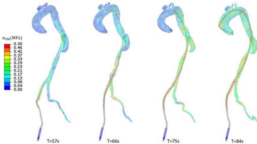
Figure 3.48: Von Mises stresses observed on the catheter during rise in the thoracic aorta at different times
