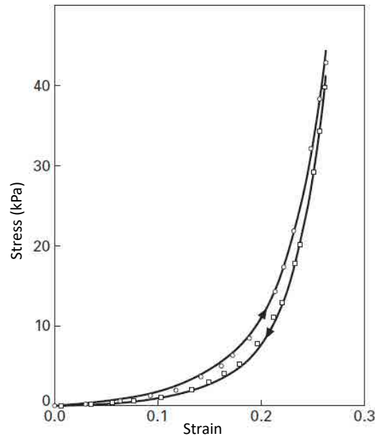
Figure 2.18: Stress-strain plots for a human vena cava sample. The circles represent loading, and the squares represent unloading (Meyers and Chawla, 2008)
