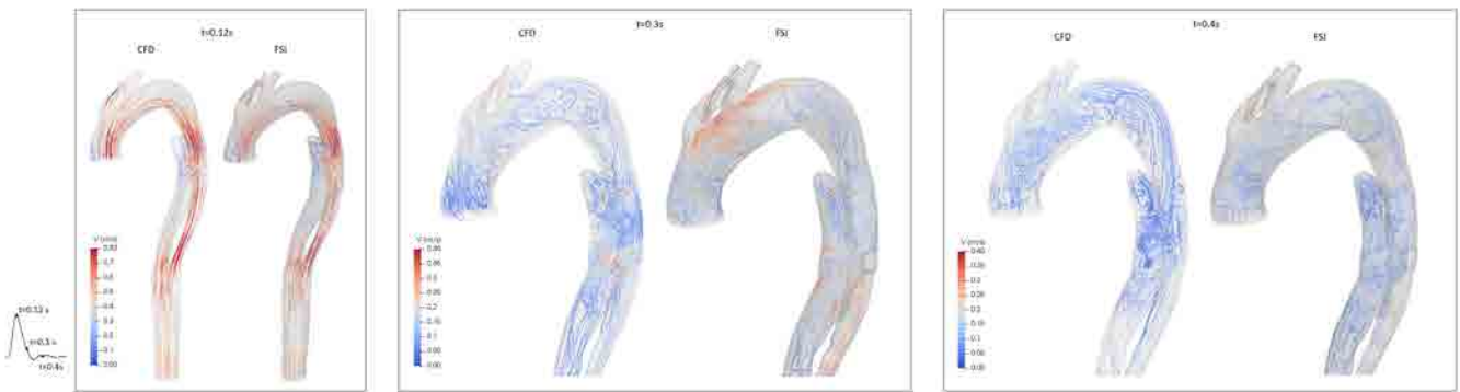
Figure 3.34: Comparison of the streamline during systole and diastole between CFD and FSI models
