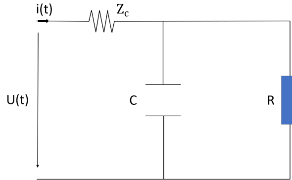
Figure 3.12: The three-element Windkessel model introduces an additional resistor Z_C connected in series with the two-element Windkessel model.
