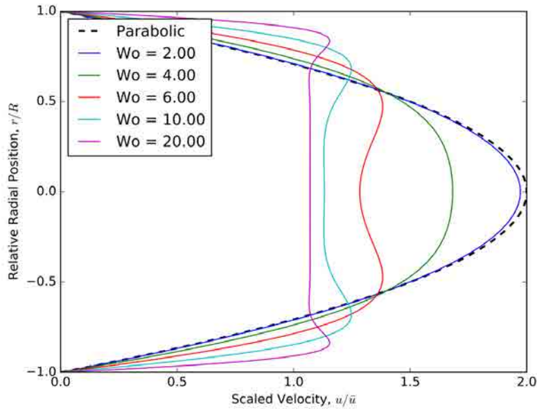
Figure 2.12: Velocity profiles for different values of the Womersley number (Hellmuth, 2017)
