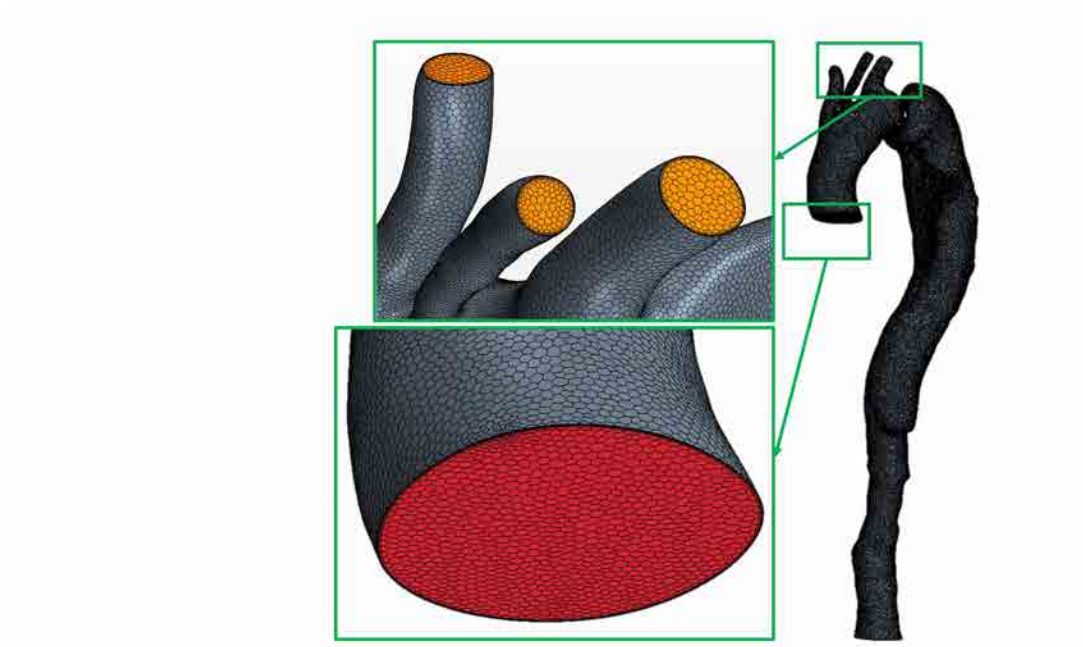
Figure 4.5: Polyhedral mesh generated with the commercial software Star-CCM+ © (1043286 cells)
