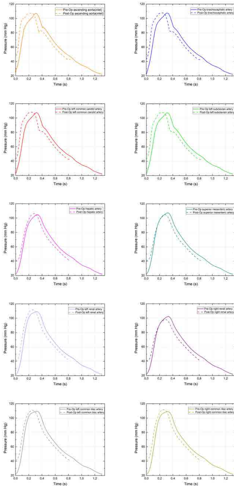
Figure 4.20: Pressure compared between the preoperative and postoperative CFD model on each boundary
