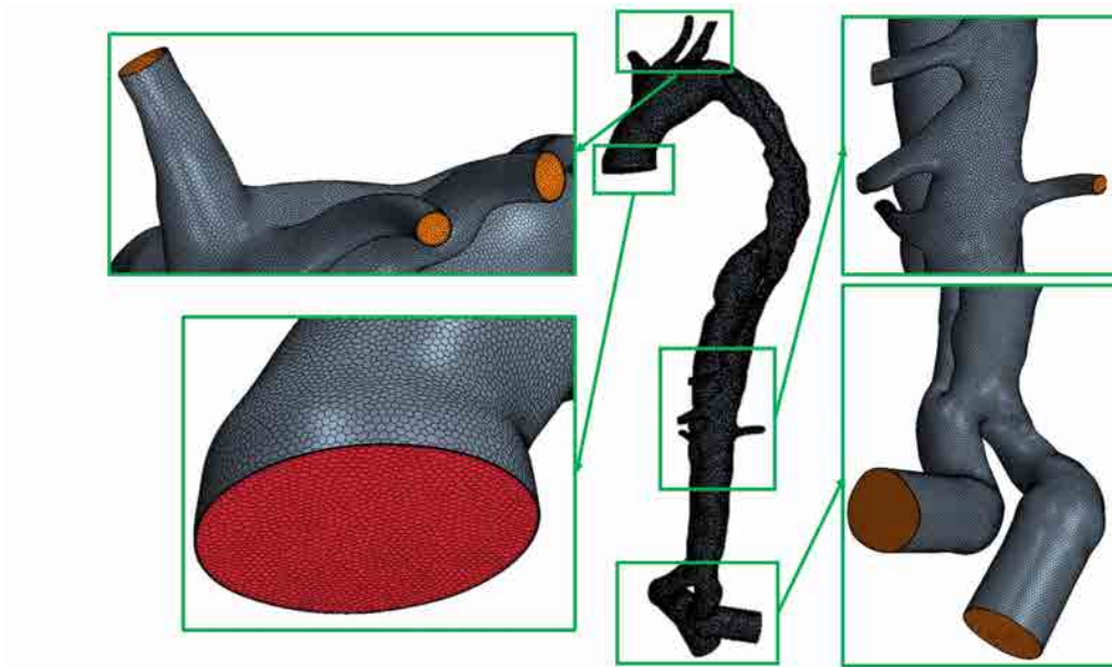
Figure 4.9: Polyhedral mesh generated with the commercial software Star-CCM+ © (1642729 cells)
