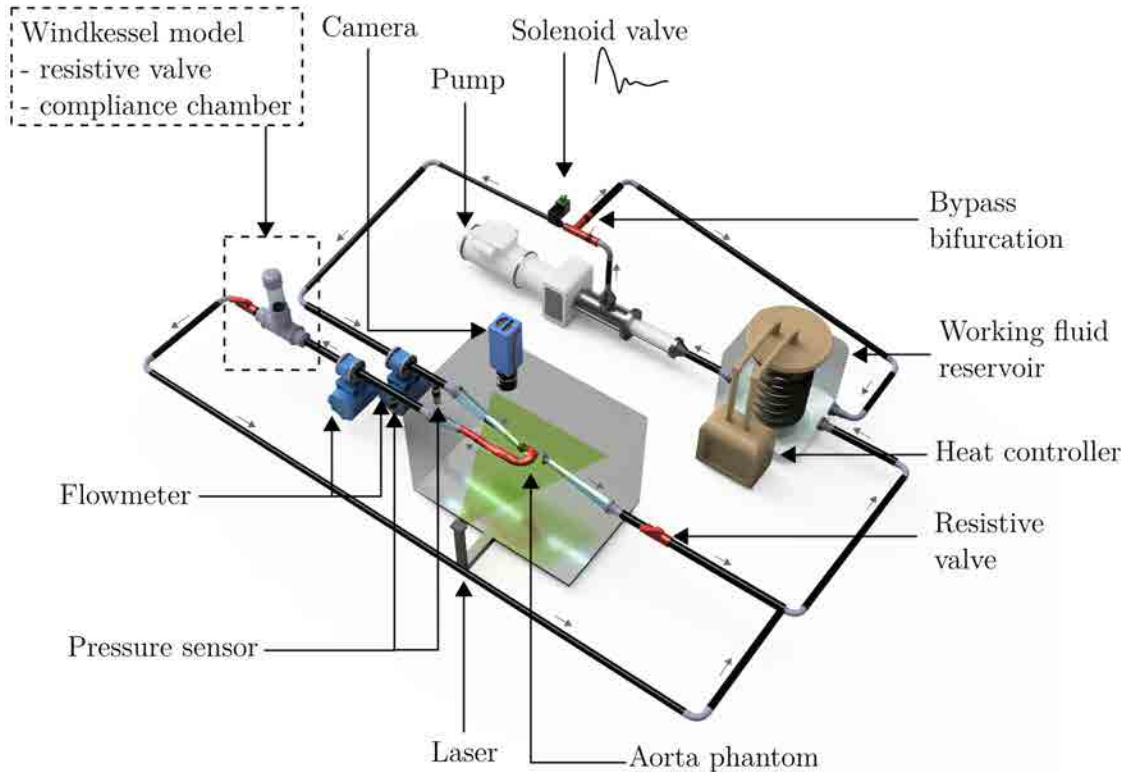
Figure 4.27: PIV experimental setup in AD configuration ((Moravia, 2021))
