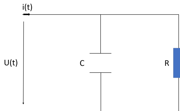
Figure 3.11: The two-element Windkessel model is analogous to the flow in an arterial system, an electrical circuit formed by a current generator, a resistor R , and a capacitor C connected in parallel.
