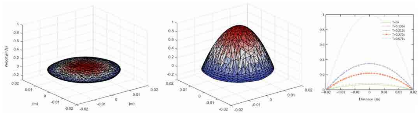
Figure 3.9: (Left) Velocity profile for a Poiseuille flow adapted to a non-circular surface at t = 0 s; (Middle) Velocity profile for a Poiseuille flow adapted to a non-circular surface at systolic; (Right) Curves of imposed velocity profiles at the entrance of the ascending aorta at different times of the cardiac cycle.
