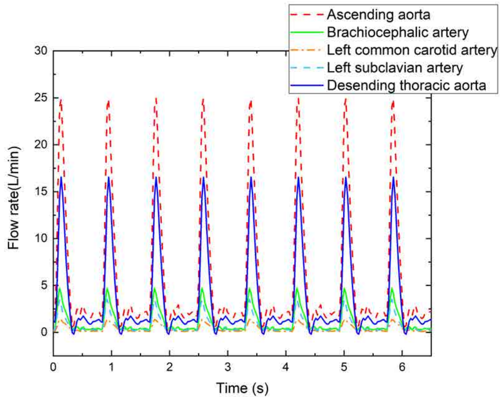
Figure 3.18: Flow rates measured with OpenFOAM over 8 cardiac cycles on the input and each output of the aorta CFD Newtonian model
