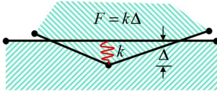
Figure 3.45: Penetration method (Menut, 2017)
