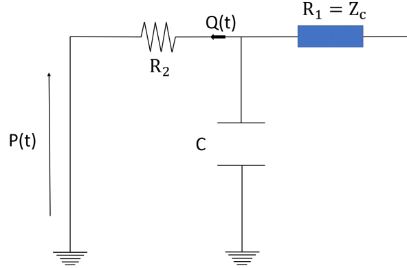
Figure 3.15: The three-element Windkessel model with the hydraulic analogy. The equation (3.7) is associated with this circuit model.
