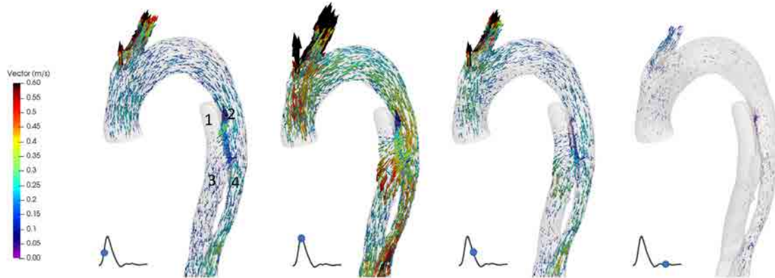
Figure 4.31: 3D observation on velocity vectors of CFD model for AD1 at four instants
