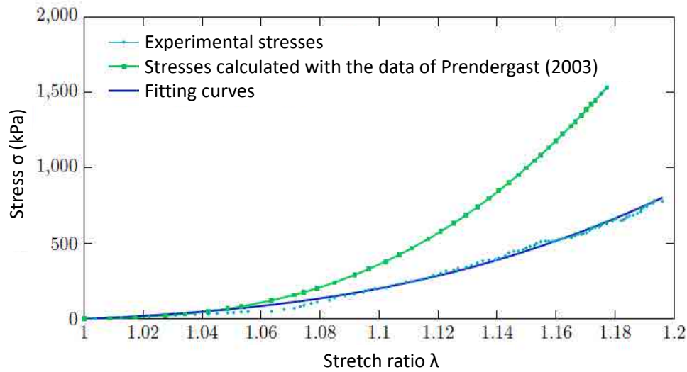
Figure 2.25: Results of swelling tests on a human aortic arch. Experimental data and fitting curves for a 5-parameter Mooney-Rivlin polynomial model (adapted from Menut (2017) )
