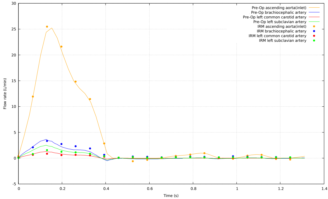
Figure 4.12: Comparison of MRI data and CFD simulation of preoperative for flow rates
