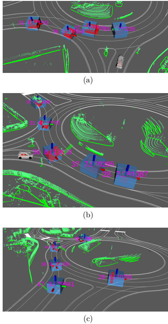
Figure 5.24: Tracked objects. The blue green and red local frame represents the pose of every tracked object, while the blue boxes represent their occupancy estimation. The LiDAR detections are in green and the corresponding curvilinear occupancy is represented by a red segment. Only the objects belonging to the drivable surface are tracked.
