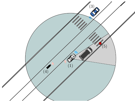
Figure 7.13: A dangerous road crossing of a pedestrian in red (5) with the field of view depicted in light blue of the white Zoe (1) partially occulted by the presence of a van (occlusion in grey).
