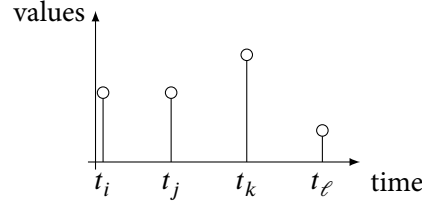
Figure 3.6: Upper/lower bound operations on an example of scheduler Q . For t_k < t < t_l the upper bound operation consists of \lceil t \rceil_Q = l . The lower bound operation consists of \lfloor t \rfloor_Q = k .
