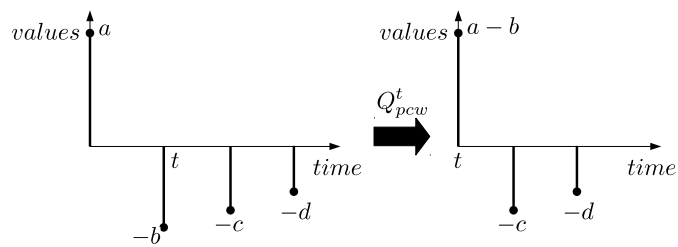
Figure 3.9: Example of piecewise prune operation Q_{pcw}^t .
