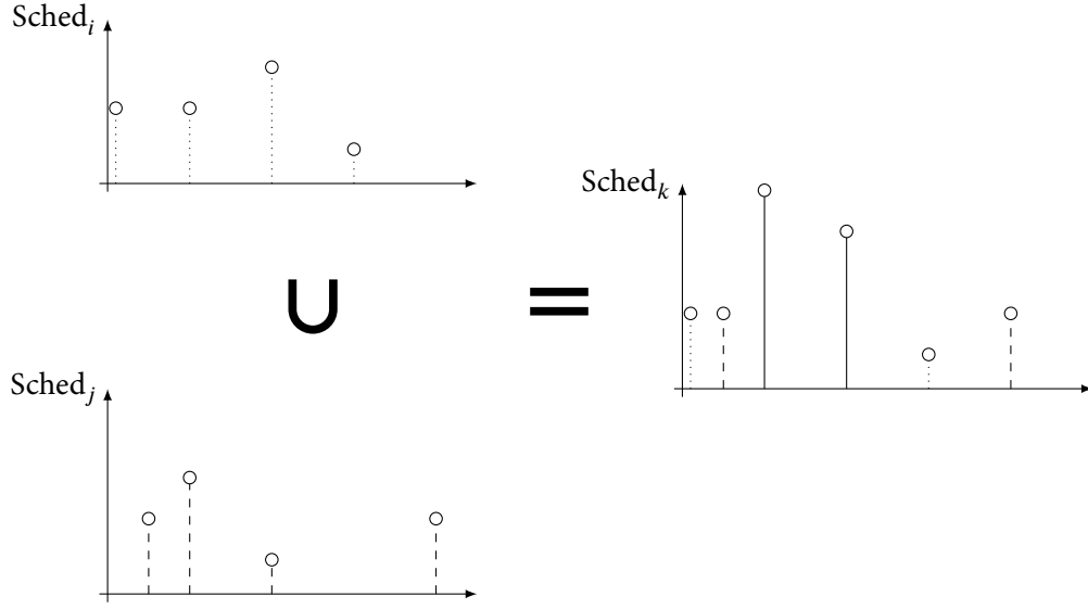
Figure 3.8: A graphical example of the union of two schedulers. The events of \text{Sched}_i are represented as dotted, while the events of \text{Sched}_j are dashed. In the merged scheduler \text{Sched}_k , the values of events at the same time in both schedulers i and j are summed and the resulting event is represented with a continuous line.
