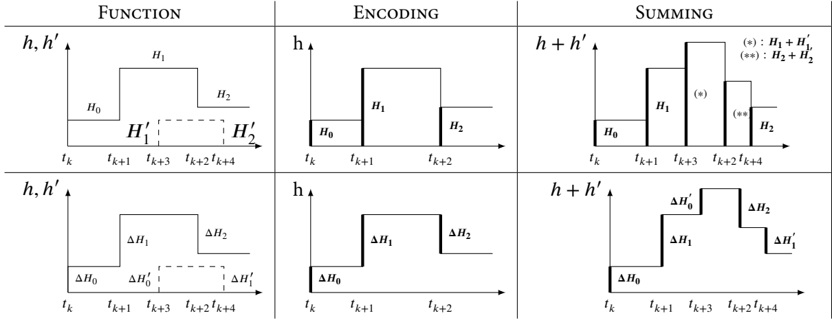
Figure 3.7: Example of a straightforward encoding of a piecewise constant function (first line) and an optimised one (second line). We use the notation H_n = h(t_{k+n}) , n \in \mathbb{N} for concision. The FUNCTION column represents the piecewise constant function h to encode (plain lines), as well as another function h' (dashed lines, see column SUMMING). Column ENCODING represents in bold the events (t_n, h(t_n)) encoded by a scheduler representing the function h . Column SUMMING represents in bold the values encoded by a scheduler now representing the function h + h' .
