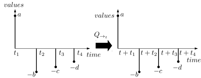
Figure 3.10: The shift operation Q_{\rightarrow t} .
