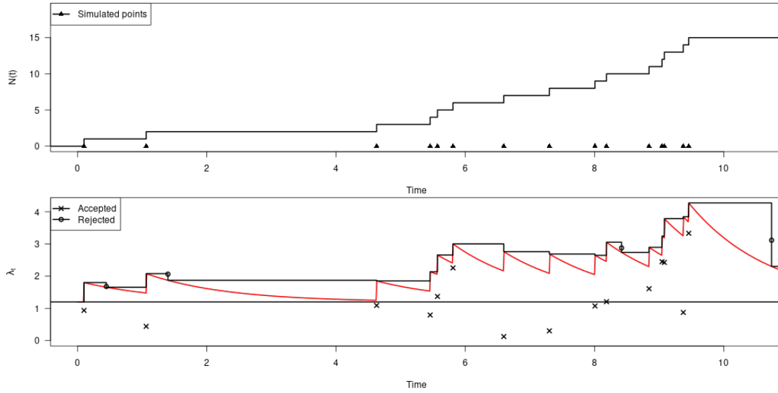
Figure 1.4: Top: A realization of a Hawkes process, represented as triangles on the bottom, with intensity function \lambda(t) = \nu + \int_0^t h(t-s) dN_s , \nu = 1.2, h(t) = 0.6 \exp -0.8t . The associated counting process N(t) is represented as well. Bottom: The intensity \lambda(t) of the Hawkes process (in red) is drawn below the constructed intensity \lambda^*(t) . The uniformly distributed values u \sim \mathcal{U}[0, 1] are displayed, by 'x' when they are accepted by the procedure, and 'o' when they are rejected.
