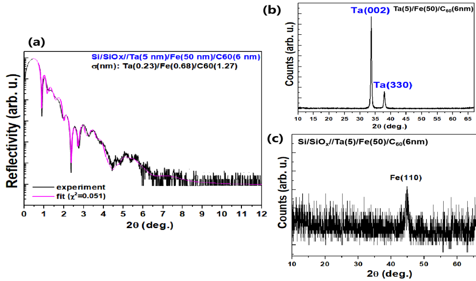
FIGURE 9.2: (a) XRR measurement on the stack Si/SiO_2//Ta(5)/Fe(50)/C_{60}(6) (nm units) with a low error fit (magenta) function \sim 0.051 that points at smooth layers in the multi-structure. (b), (c) the XRD patterns for tantalum and iron. A strong diffraction peak at (002) is seen for Ta accompanied by a minor peak at (330). For iron a peak at \sim 45^\circ is for bcc(110) structure for Fe sputtered on Ta buffer.
