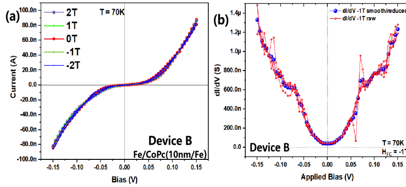
FIGURE 8.14: Magnetotransport on Device-B : Fe/CoPc(10nm)/Fe. (a) Non-linear, Ohmic IV at 70K for almost in-plane magnetic field values. (b) Bias dependence of conductance curve exhibits flat region then sudden jumps with increasing bias values signature of spin-flip excitations.
