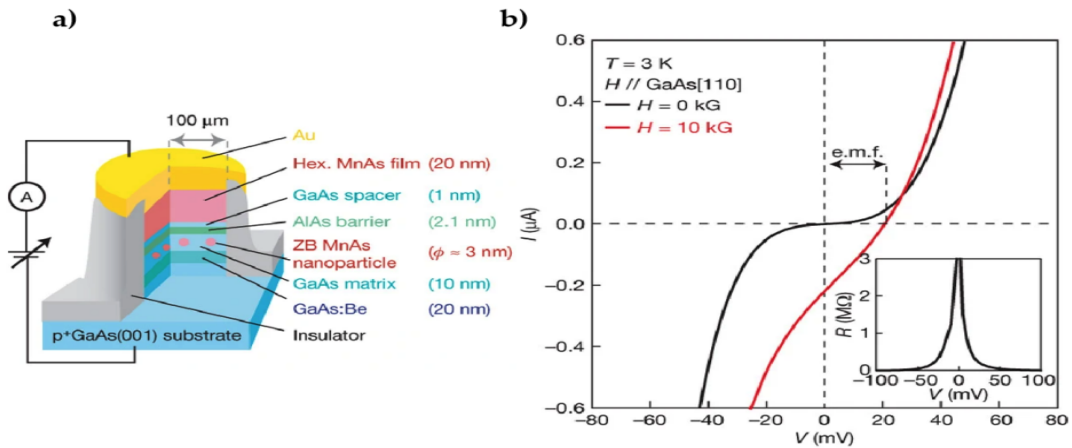
FIGURE 4.6: Spin Battery. (a) MTJ structure. (b) Current vs voltage plot measured at T = 3\text{K} without (black) and with (red) \mathbf{H} = 1\text{T} applied in-plane to GaAs[110]. In the presence of a magnetic field a positive current is induced for a negative voltage bias. Inset gives the MTJs resistance sweep for V = \pm 100\text{mV} at \mathbf{H} = 0\text{T} and 50\text{meV} of Coulomb blockade was observed. Image taken from Ref [13].
