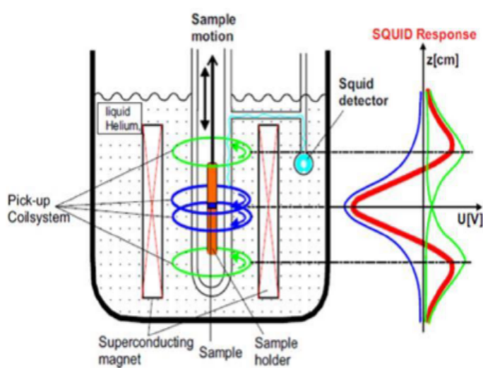
FIGURE 5.9: SQUID set-up. The best position for optimum SQUID output voltage is recorded for the sample is when it is in between the blue colored pick up coils. The figure is adopted from Ref [120].
