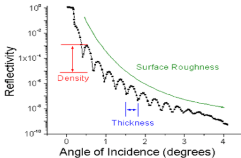
FIGURE 5.11: X-ray reflectometry of a thin-film. From the graph, slope gives the surface roughness ; drop in signal determines the density of the material and the distance between the fringes gives the thickness of the thin film. Figure adapted from Ref [199].
