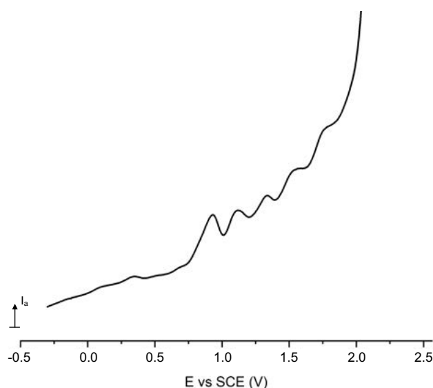
Figure 18. Square wave voltammogram of ([\text{RuPMe}]_n\text{-RuNPs})^+(\text{PF}_6^-)_n in solution.
