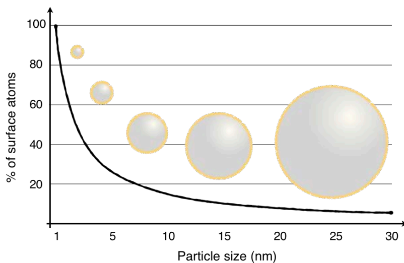
Figure 3. Surface/bulk atomic ratios as a function of particle size.
