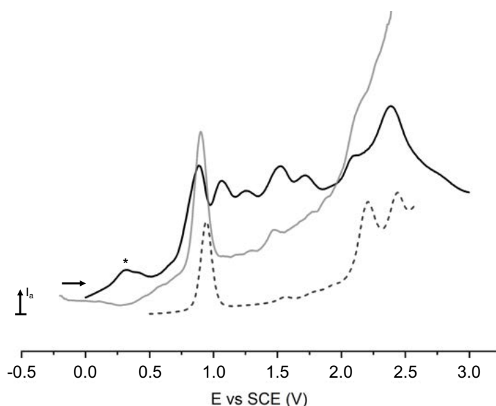
Figure 11. Square wave voltammogram of the oxidation of ([RuPMe] n -RuNPs) + (PF 6 - ) n (black), [RuPMe] + PF 6 - (grey) deposited on the GC electrode and [RuPMe] + PF 6 - in solution (dashed).
