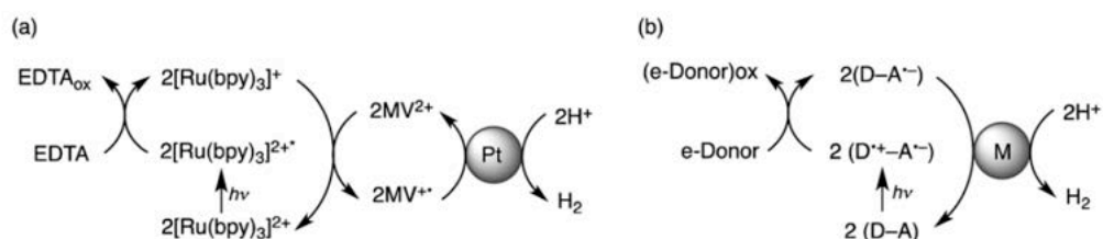
Figure 22. Catalytic cycle of (a) a conventional reaction system constructed by EDTA, [\text{Ru}(\text{bpy})_3]^{2+} , \text{MV}^{2+} and PtNPs and (b) donor-acceptor linked dyad without electron mediator ( \text{M} = \text{Ru} ). Reproduced from [42].
