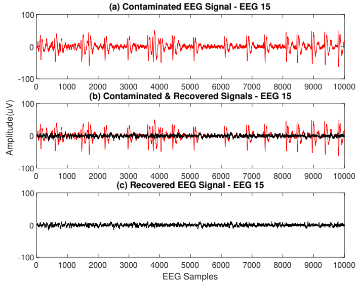
FIGURE 5.7 – Recovered EEG signal through proposed FastEMD-CCA 2
