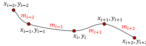
FIGURE 3.2 – Slope computation at point [x_i, y_i]
