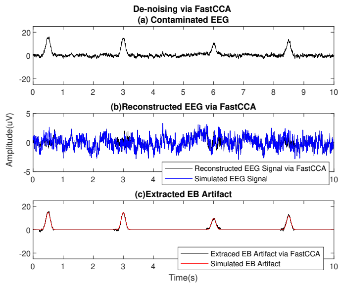
FIGURE 5.2 – (a) Mixed EEG and Eyeblink Signal, (b) Reconstructed EEG Signal, (c) Extracted Eyeblink Artifact
