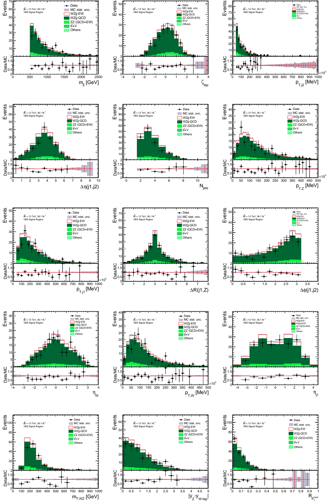
Figure 5.4: Control distributions of the BDT inputs in the Signal region. No correction of the MC distributions normalisations is applied.
