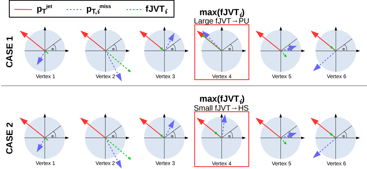
Figure 4.3: Schematic representation of the fJVT jet-tagging process, for a six-vertices event. Top row illustrates the case of a PU-like forward jet, while bottom row illustrates the HS-like forward jet case.
