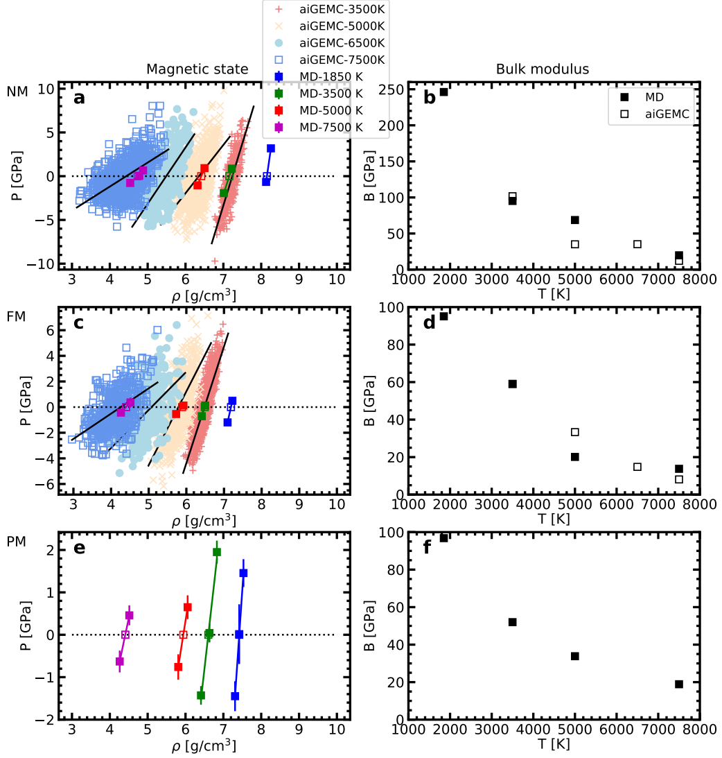
Figure 5.4: (a) The pressure-density fluctuation in the ai GEMC simulations for iron in the nonmagnetic (NM) and ferromagnetic state (FM) at 3500, 5000, 6500 and 7500 K. (b) The bulk modulus of the liquid iron phase defined as \rho \frac{dP}{d\rho} , where \frac{dP}{d\rho} is derived by a linear fitting of the pressure-density data. In comparison, we also performed ai MD simulations for the liquid iron in the nonmagnetic, ferromagnetic and paramagnetic state (PM) to find the zero pressure density and estimate its bulk modulus.
