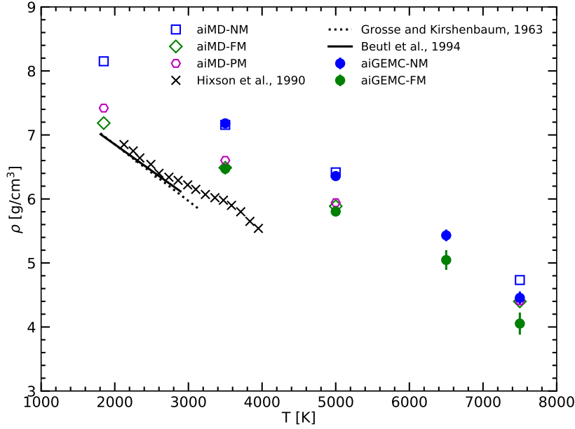
Figure 5.5: The zero pressure density up to 7500 K obtained from ab initio MD simulations. For comparison, we also plot the equilibrium liquid iron density derived from aiGEMC simulations and experimentally determined liquid iron density at around 0 GPa (Beutl et al., 1994; Grosse and Kirshenbaum, 1963; Hixson et al., 1990).
