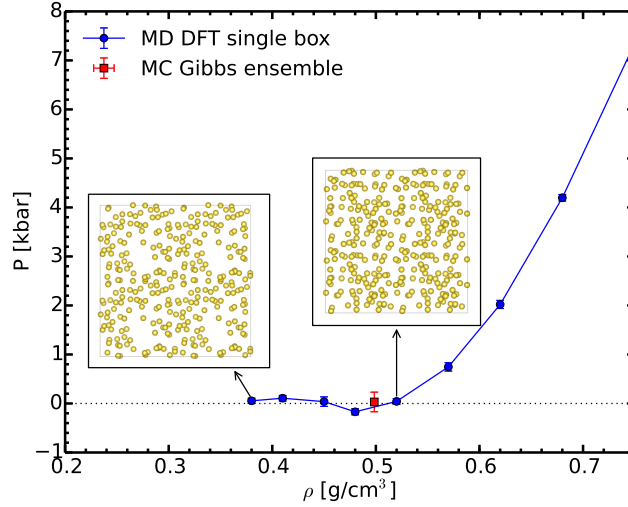
Figure 4.5: Pressure evolution during the isothermal volume expansion for sodium at 2000 K. The insets show the snapshots at 0.52 and 0.38 g/cm 3 , respectively.
