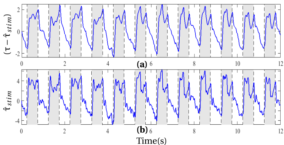
Figure 5.15: Control torque when FES is enabled: (a) Motor torque ( \tau - \hat{\tau}_{stim} ), (b) Estimated stimulation torque ( \hat{\tau}_{stim} ). The grey bars represent the knee joint extension phases when FES is enabled.
