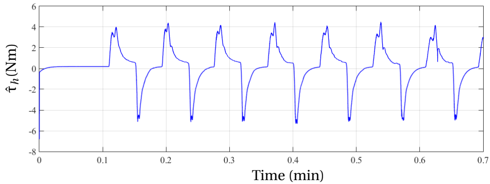
Figure 7.4: Estimated knee joint torque \hat{\tau}_h when using only FES.
