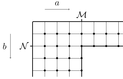
Fig. 8.1 The H_{m|n} domain for \mathscr{A}(\mathfrak{gl}(m|n)) fusion
