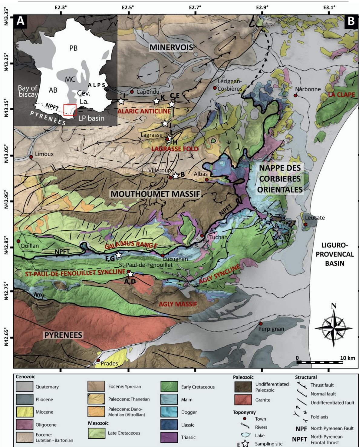
Figure IV-2 - Location of the study area and sampling sites. (a) Red square: studied area in the North foreland of the East Pyrenean belt (Corbières domain). PB, Paris basin; AB, Aquitaine basin; MC, Massif Central; Cév., Cévennes; La., Languedoc. (b) Structural scheme and sampling sites (white stars). Modified using 1/50,000 and 1/80,000 BRGM geological maps
