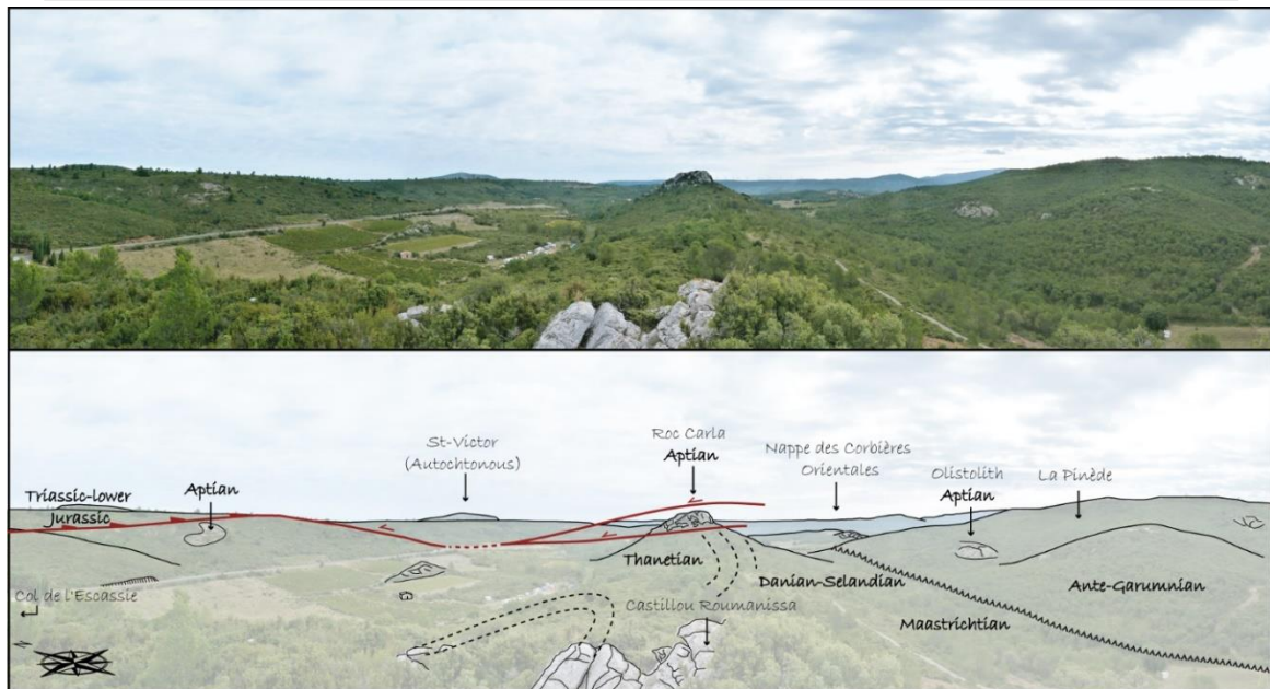
Figure IV-13 - View and interpretation of the "Roc Carla" looking east from Castillou-Roumanissa hill showing the NW progression of the NCO and the overturning of its footwall. The "Roc Carla" is interpreted as an Aptian block dragged at the base of the NCO.
