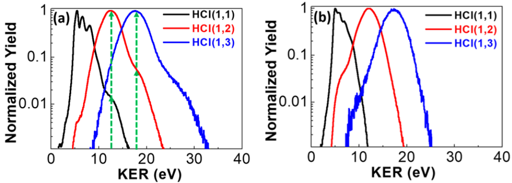
Figure 3.3 (a) The KER spectra of the HCl (1,q) ( q=1, 2, and 3 ) channels in linearly polarized laser field. (b) The same to (a) but for circular polarization.
