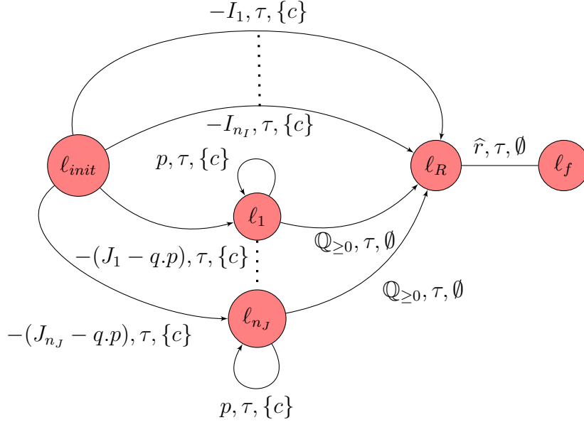
Figure 4.15: An automaton using T to encode the closure in \ell_f .
