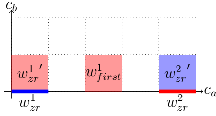
Figure 5.19: Binary search between enlarged zones.
