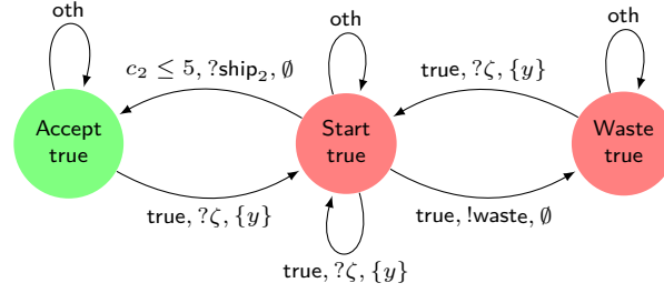
Figure 3.6: A test purpose for the conveyor belt.
