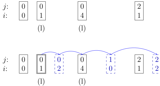
Figure 3.13: An execution of updateRank
