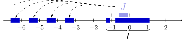
Figure 4.5: Example of a regular union of intervals.
