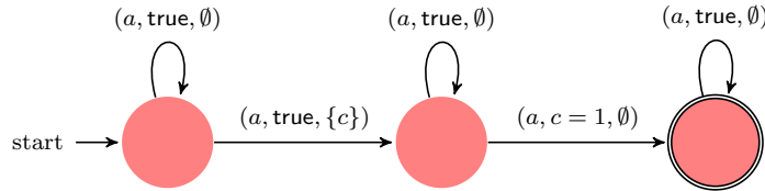
Figure 5.1: A one-clock non-determinizable RERA.
