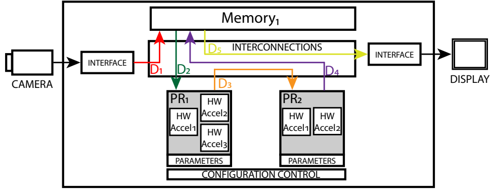
Figure 3.36 – SPS-CGRA example 8
