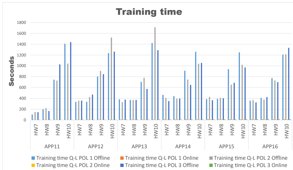
Figure 8.12 – Training time of the Q-learning approaches.
