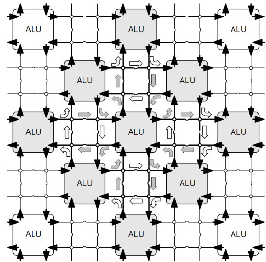
Figure 1.6 – CHESS layout [2].
