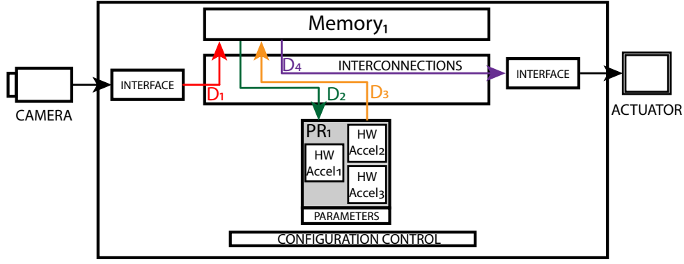
Figure 3.27 – SPS-CGRA example 4
