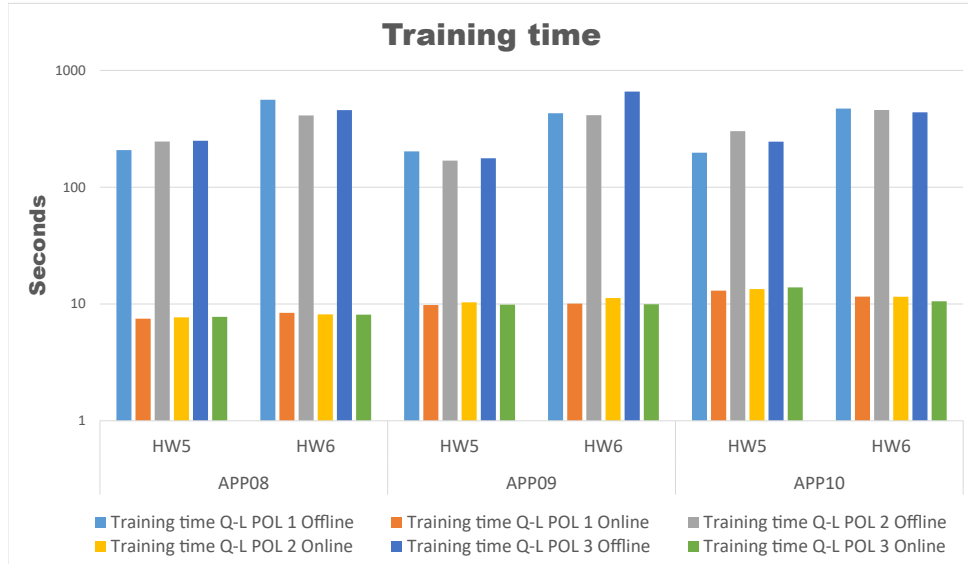
Figure 8.8 – Training time of the Q-learning approaches.
