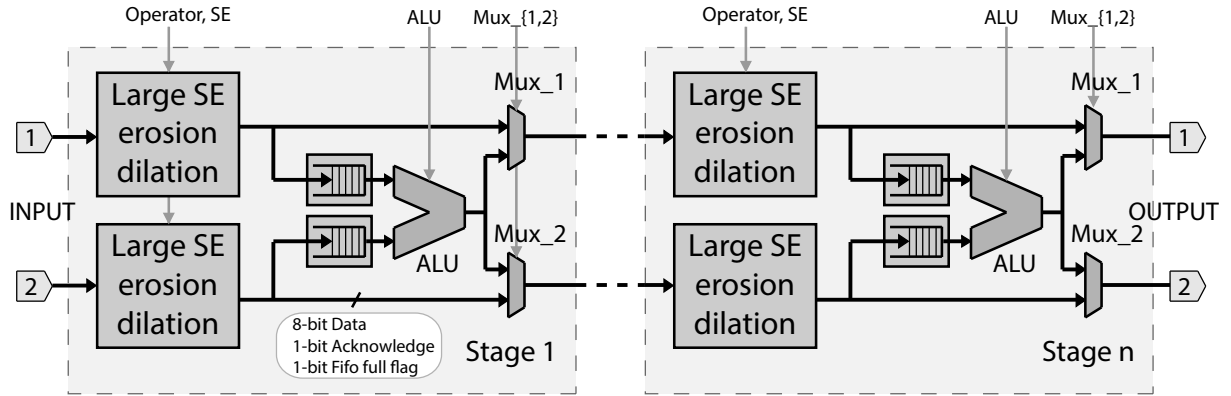
Figure 3.40 – Large SE pipeline architecture
