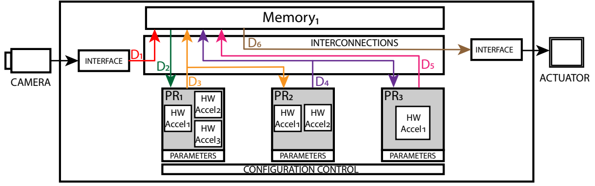
Figure 3.25 – SPS-CGRA example 3
