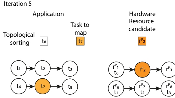
Figure 6.21 – Fifth iteration of example 2.
