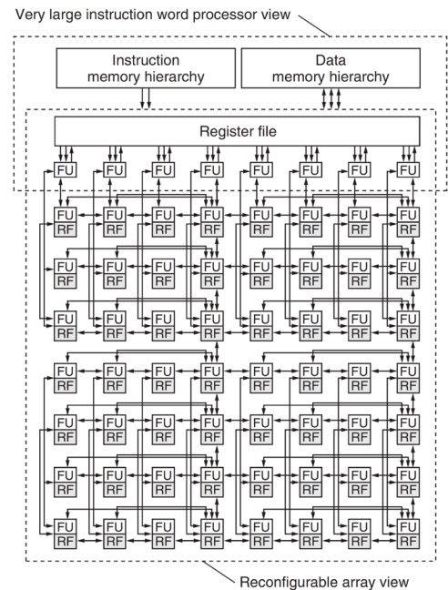
Figure 1.10 – ADRES interconnection [4, 5].
