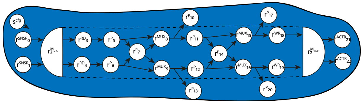
Figure 3.41 – Hardware model of the MCPU
