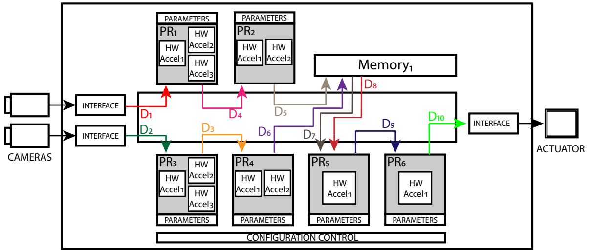
Figure 3.33 – SPS-CGRA example 7
