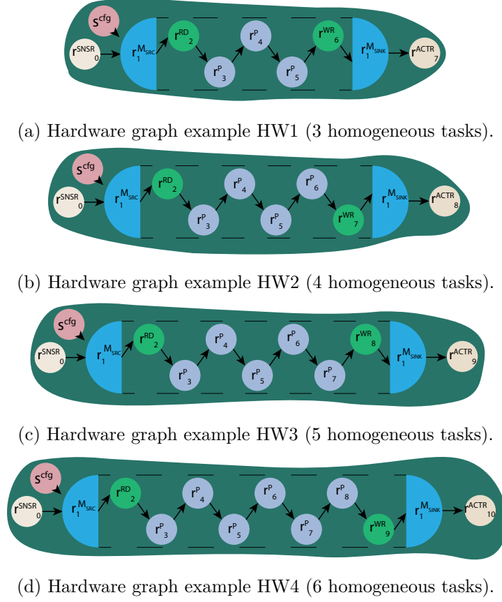
Figure 8.2 – First set of hardware examples
