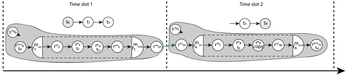
Figure 4.4 – Inclusion of the data dependency resources between time slots
