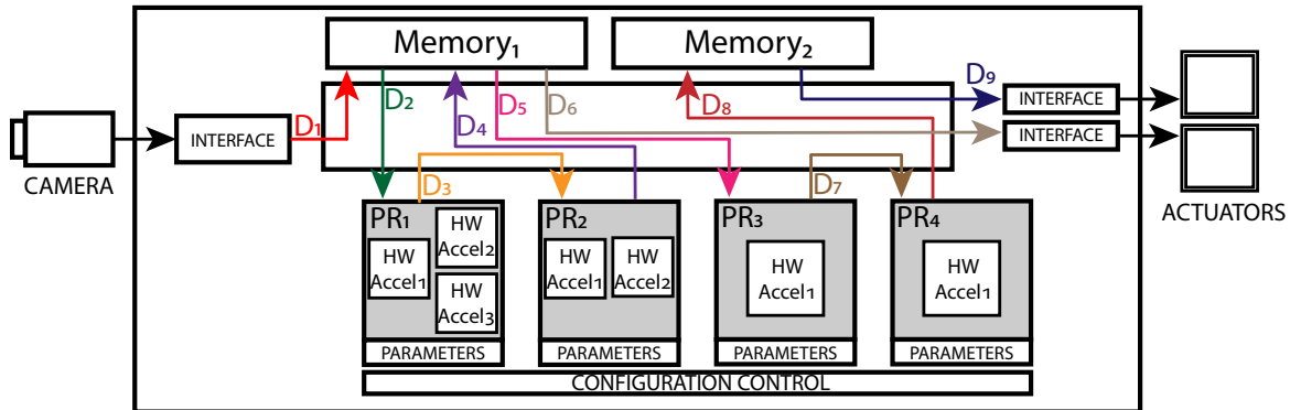
Figure 3.31 – SPS-CGRA example 6
