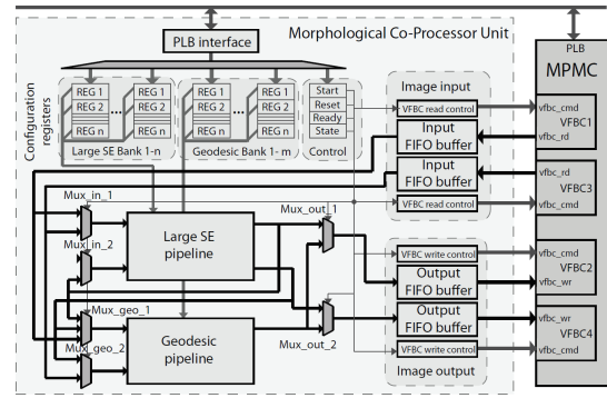
Figure 1.18 – Architecture of the MCPU [12].
