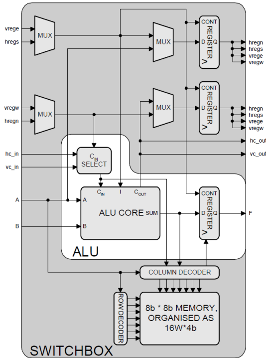
Figure 1.5 – Logical structure of a CHESS processing element [2].
