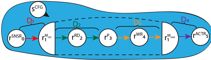
Figure 3.28 – Hardware model of example 4
