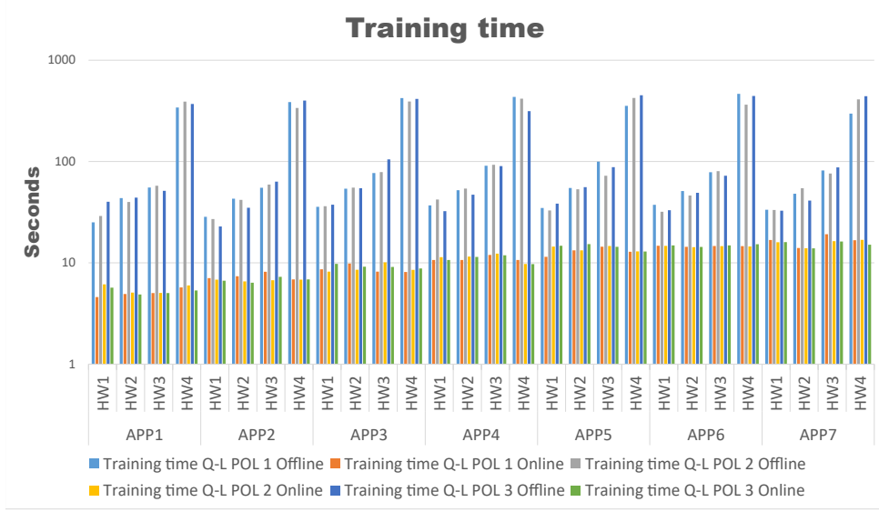
Figure 8.4 – Training time of the Q-learning approaches.
