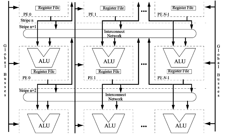
Figure 1.12 – PipeRench interconnection [6, 7].
