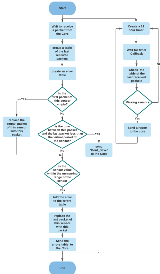
Figure 1.12 The flowchart of the detection module
