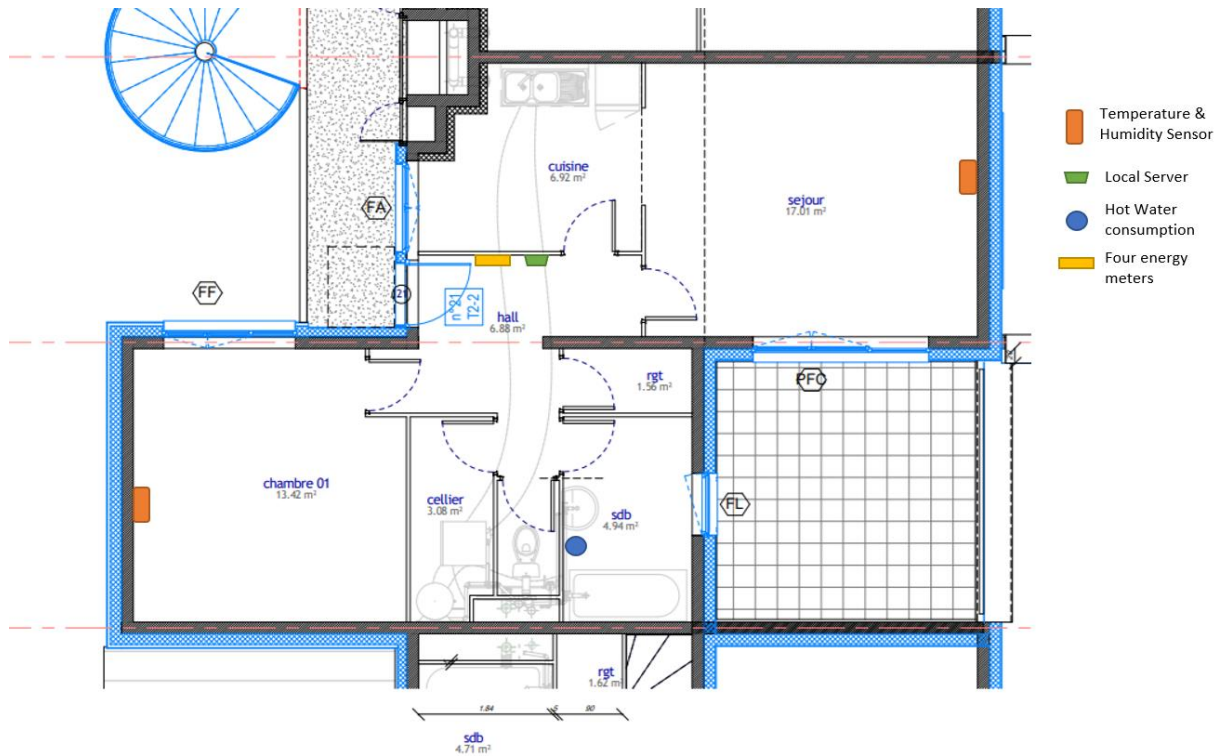
Figure 1.2 Instrumented Building
