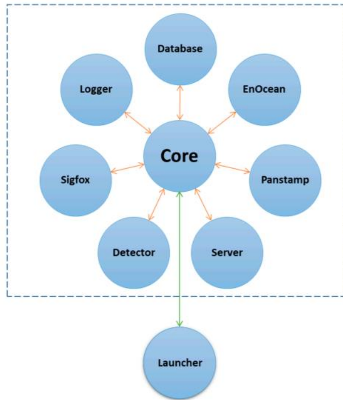
Figure 1.8 Software modules
