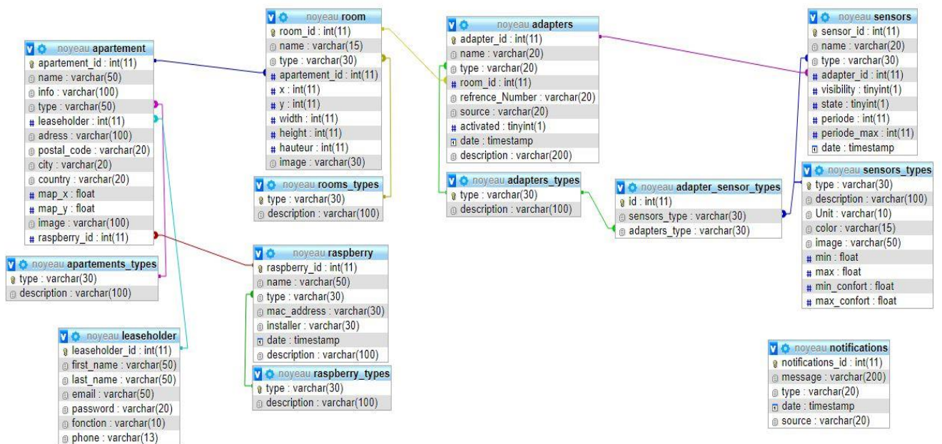
Figure 1.7 Database structure
