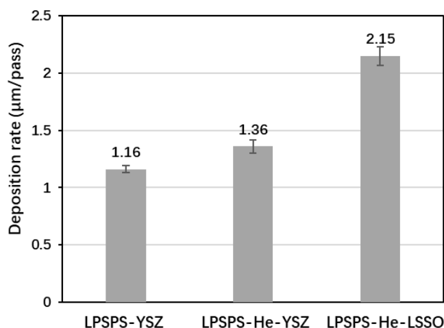
Fig. 5.7 Deposition rate of the electrolytes
