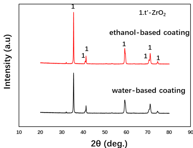
Fig. 4.23 XRD patterns of LSPS YSZ coatings prepared with different suspension solvents
