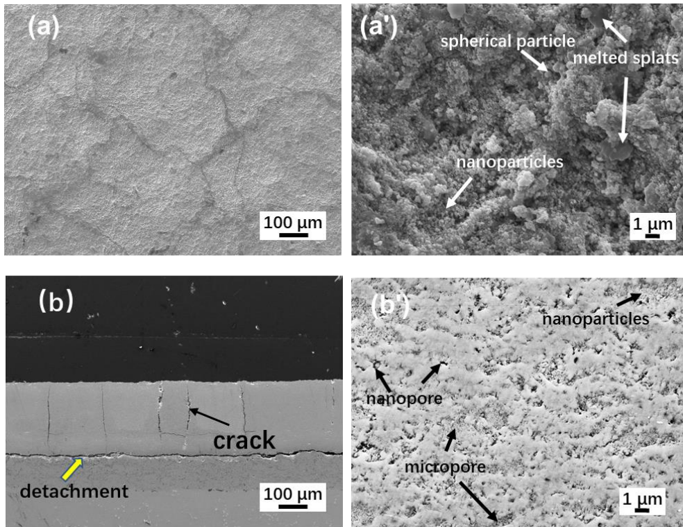
Fig. 4.2 SEM images of LSPSP YSZ coating prepared in the argon: (a)(a') surface morphologies, (b)(b') cross-sectional morphologies
