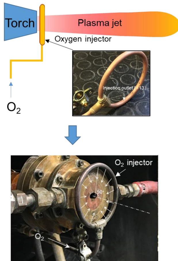
Fig. 4.11 The form of oxygen injection into the plasm jet
