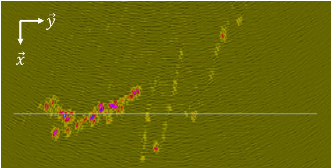
Fig. 61. Recorded image using FMC/TFM imaging of the cracks represented in fig. 1.
