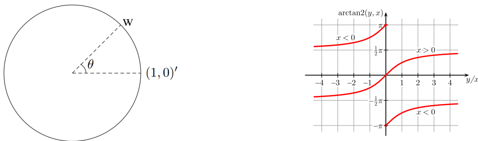
Figure 3.1: An illustration for the definition of the function (y, x) \mapsto \text{atan2}(y, x) .
