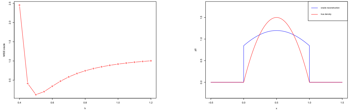
(a) Plots of h \mapsto \text{MISE}_{\text{oracle}}(h) for the Beta(2,2) density p_0
