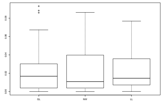
(b) Boxplot of pointwise squared risk in comparison with NW and LL
