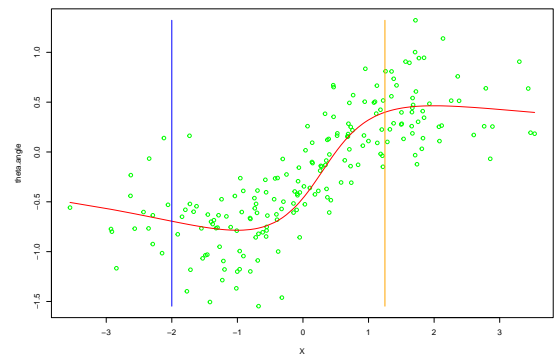
(b) Model M1 : X_j \sim \mathcal{N}(0, 1.5)
