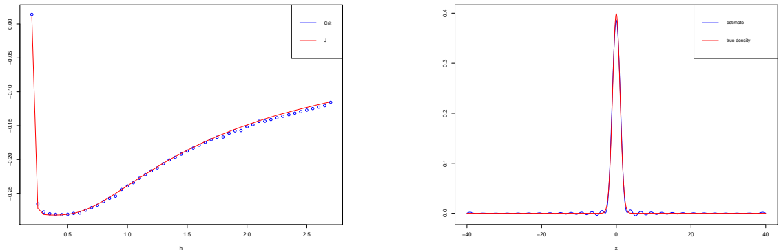
(a) Plots of h \mapsto \text{Crit}(h) and h \mapsto J(h) for Gaussian density p_0
