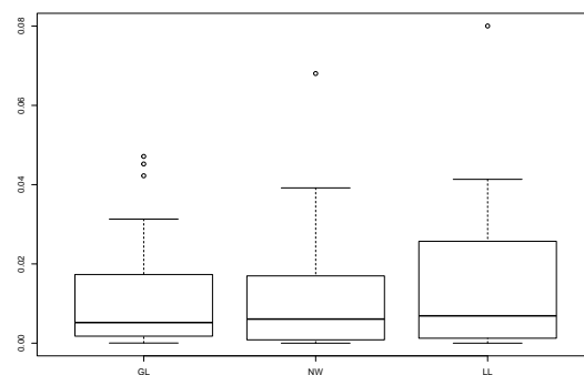
(b) Model M3: estimation at x = 0.95 with X \sim U([0, 1]) .
