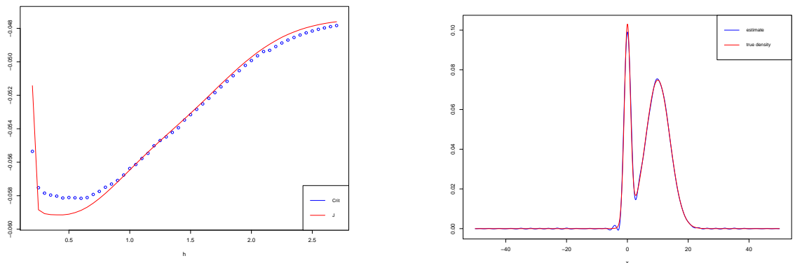
(a) Plots of h \mapsto \text{Crit}(h) and h \mapsto J(h) for the Gaussian mixture density p_0
