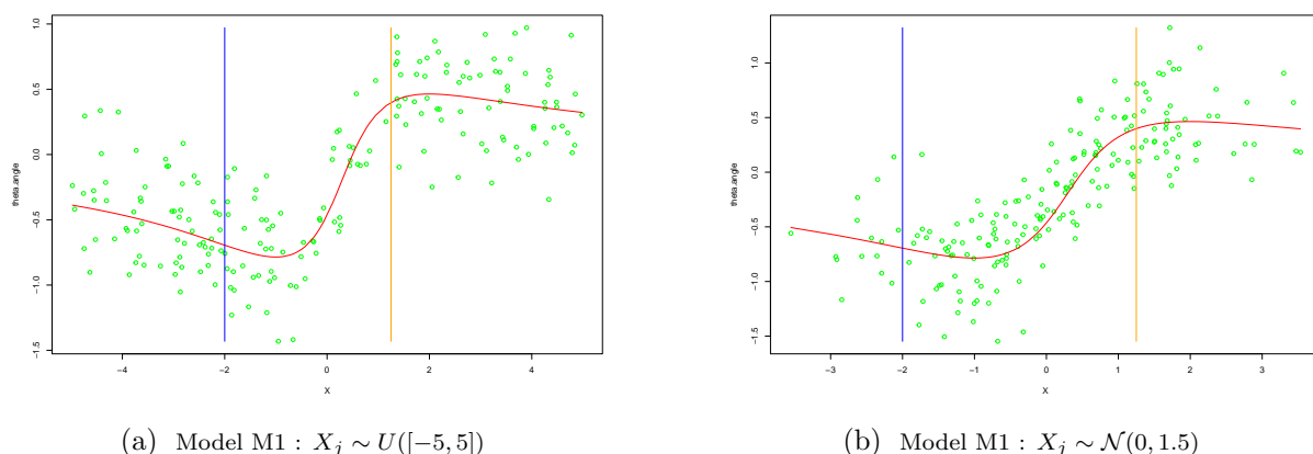
Figure 1.2: An illustration for simulated data \{\Theta_j\}_{j=1}^n (green points) of model-M1 with n = 200 . The red curve presents the true regression function m , while the blue vertical line displays point x = -2 and the orange vertical line displays point x = 1.25 where we aim at estimating m(x) .
