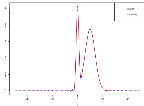
(b) \mu_0 \sim Y \times \mathcal{N}(0,1) + (1 - Y) \times \mathcal{N}(10,4) with Y \sim \text{Bernoulli}(0.25)
