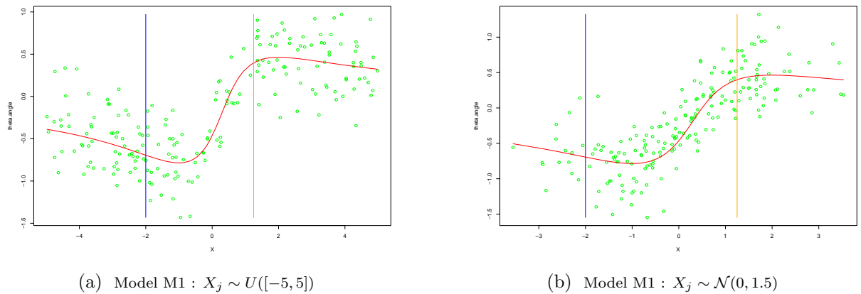
Figure 3.4: An illustration for simulated data \{\Theta_j\}_{j=1}^n (green points) of model-M1 with n = 200 . The red curve presents the regression function m , while the blue vertical line displays point x = -2 and the orange vertical line displays point x = 1.25 where we aim at estimating m(x) .
