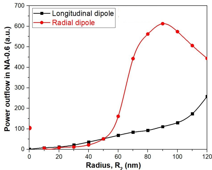
Figure 2.13: Comparison between the effect of NW radius on the power collected in NA 0.6 for a radial dipole (red) and longitudinal dipole (black). The dipole position and tapering half-angle \theta/2 are fixed at 100 nm and 2^\circ respectively.
