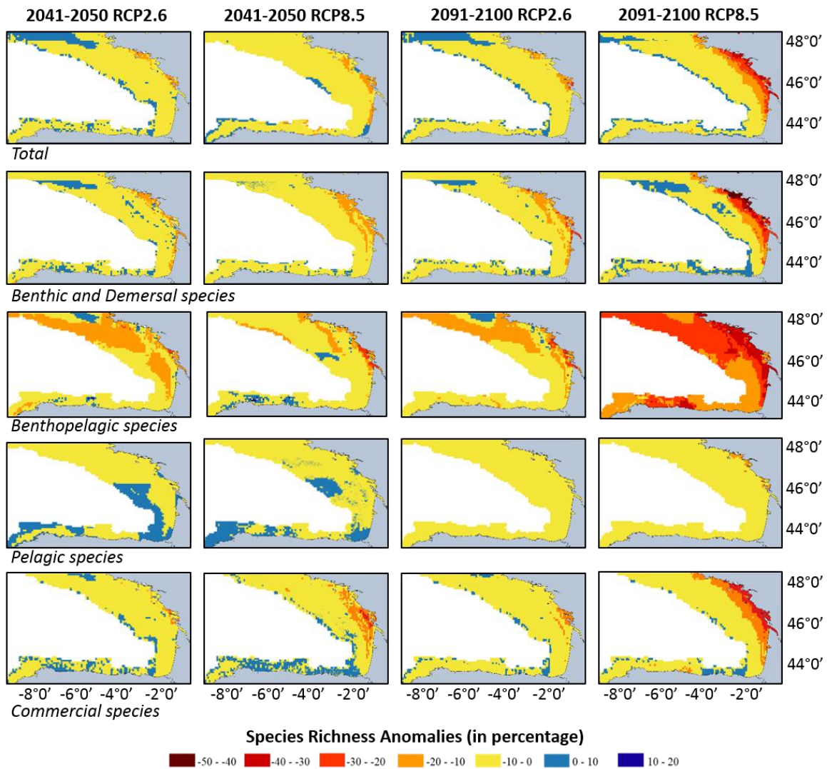
Figure 2: Projected species richness anomalies (percentage) in the Bay of Biscay for all species ( n = 163 ), bottom species ( n = 41 ); benthopelagic species ( n = 83 ); pelagic species ( n = 39 ) and commercial species ( n = 73 ) under each scenario and period compared with current species richness. Warm colors represent a decrease in species richness and the cold colors represent an increase in specific richness.
