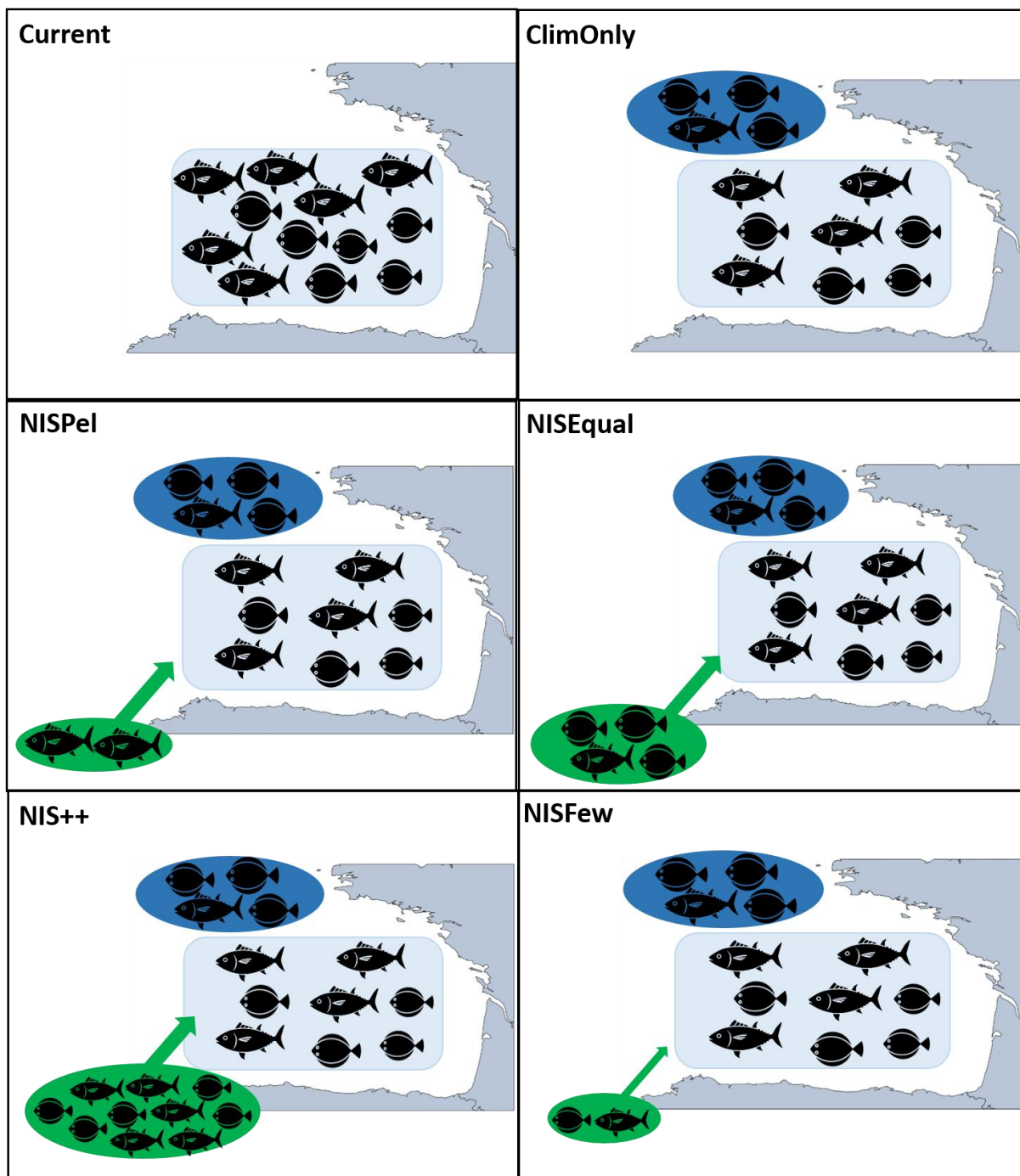
Figure 2: Diagram of the current model (2007-2016) and the 5 projected scenarii (2041-2050). The blue shapes represent the Bay of Biscay species (light blue for species not impacted by climate change and deep blue for species with a reduced biomass due to climate change). The green shapes represent the non-indigenous species (NIS). Tuna shape represents the pelagic and benthopelagic species, flatfish shape represents the benthic and demersal species. The size of the green circle is function of the NIS biomass.
