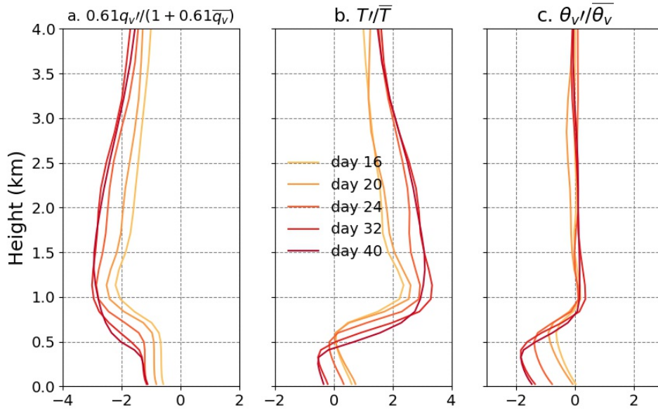
Figure 4.4: Plots show the contribution of a) q_v anomalies and b) temperature anomalies into c) virtual potential temperature anomalies. Each line is one day averaged over the dry patch ( CRH < 0.6 ) for the simulation H5SST305.
