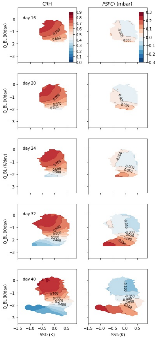
Figure 4.5: CRH (left column) and PSFC anomaly (right column) for simulation H5SST305. The x axis is SST anomaly, and the y axis is radiative cooling averaged over the boundary layer Q_{BL} . To compute the top of the boundary layer, we use the q_v profile and determine the first altitude above ground where it has a maximum curvature.
