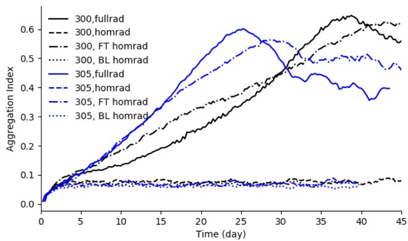
Figure 4.12: Plot shows the aggregation index time series for the sensitivity tests at 300K (black curves) and 305 K(blue curves). Homrad, FT and BL stand for homogenized radiation, free troposphere and boundary layer respectively.
