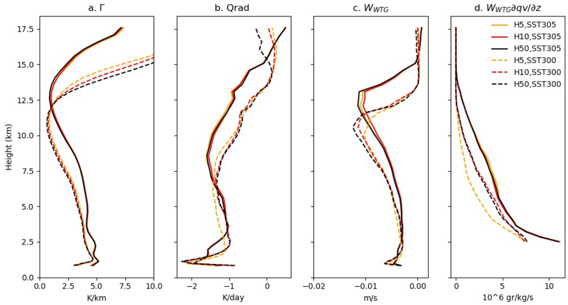
Figure 4.10: Plot shows: a) the stratification, b) atmospheric radiative cooling, c) vertical velocity computed by WTG, and c) dryness tendency. The variables are averaged over transient part ( 0.2 < \delta CRH < 0.5 in Figure 4.1)
