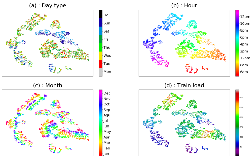
Figure 3.14.: Latent representation ( u_t ) according to contextual features with dimension reduction
