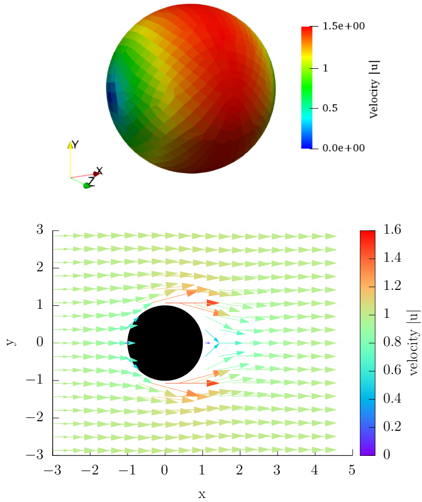
FIGURE 2.10: Demonstration of the velocity field resulting of an obstacle sphere in a potential flow, displayed on a section of the surrounding flow and at the centers of the sphere mesh faces.
