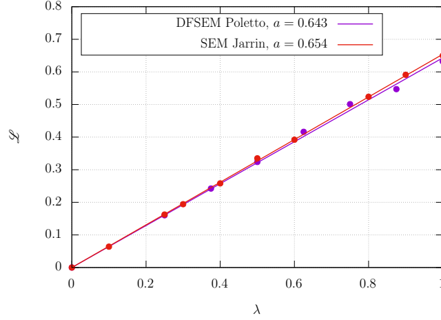
FIGURE 4.6: Taylor macro-scale versus length scale \lambda , I_\infty = 15\% , U_\infty = 1.0 m/s, \sigma(\lambda) = 0\% , R_f = 1 .
