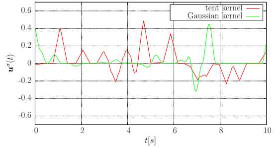
FIGURE 3.12: Temporal measurements of velocity fluctuations u^\sigma(t) at one point, for different kernel functions f_\lambda (with I_\infty = 15\% , \lambda = 0.25 , \sigma(\lambda) = 25\% , R_f = 1 ).
