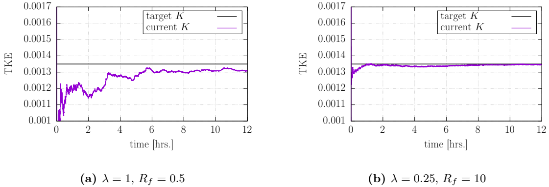
FIGURE 3.8: Time series of the current values of the TKE K computed at a single point over 12 hours of simulated time, for the low turbulence intensity I_\infty = 3\% . On the left : an example of very slow convergence, with few turbulent structures of large size \lambda . On the right : an example of fast convergence, with a high saturation R_f of structures of small size \lambda .
