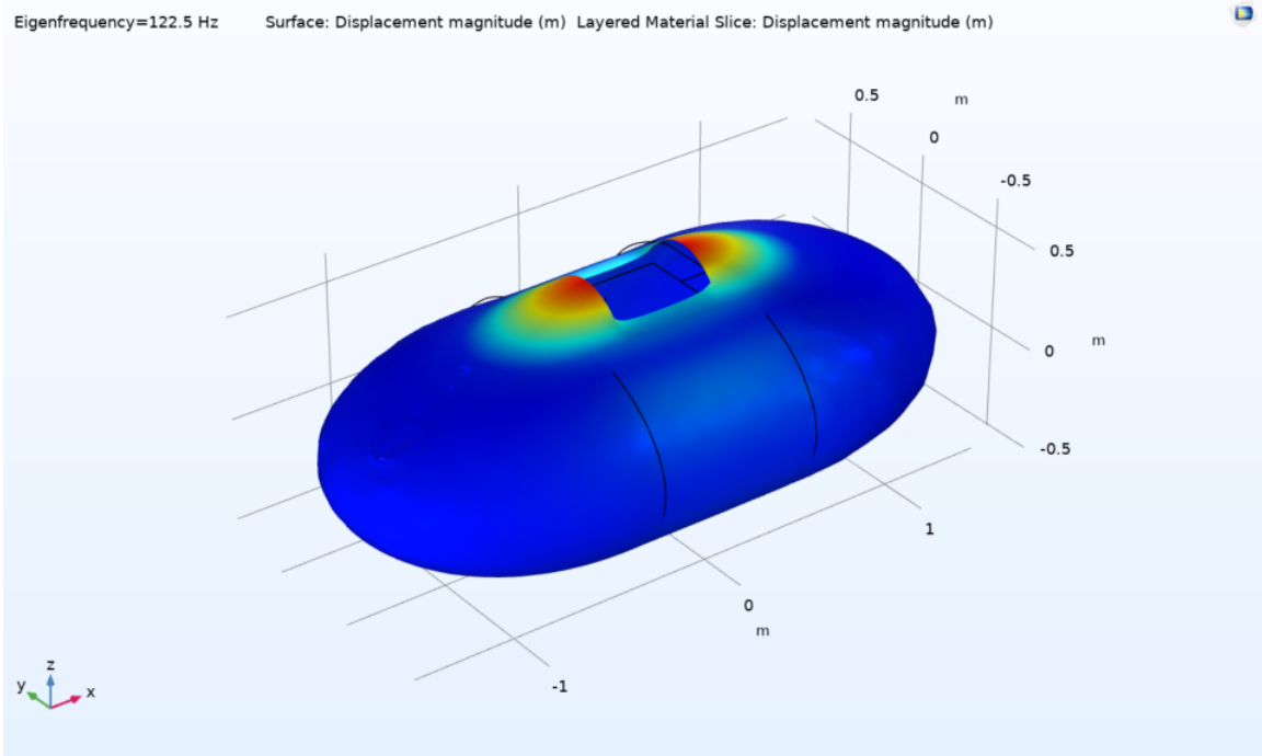
Figure 3.19: Sixth flexural mode of the system ogive-test panel, in comparison with the first flexural mode of just the ogive.
