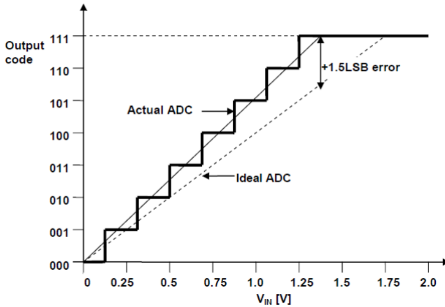
Figure 2.5: Example of the gain error, extracted from [7].
