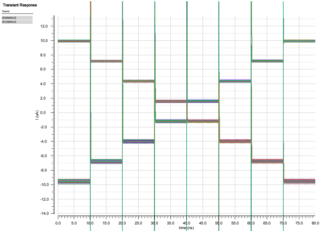
Figure 4.32: The transient response of the proposed feedback DAC through Monte-Carlo simulations.
