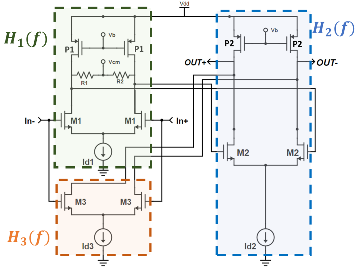
Figure 4.6: Simplified schematic of the proposed two-stages NCFE opamp.
