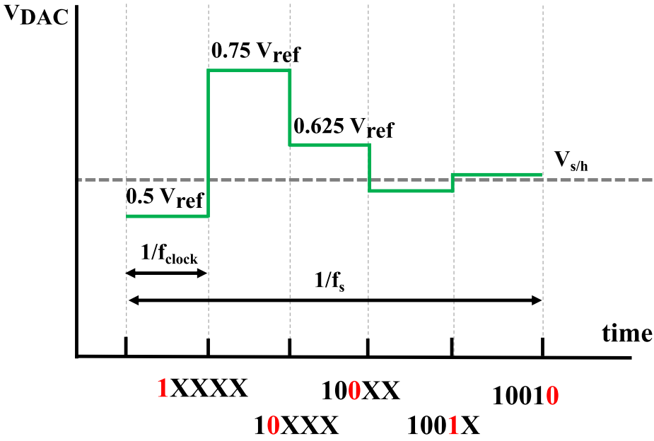
Figure 2.11: Exemple of an approximation sequence of a SAR ADC.
