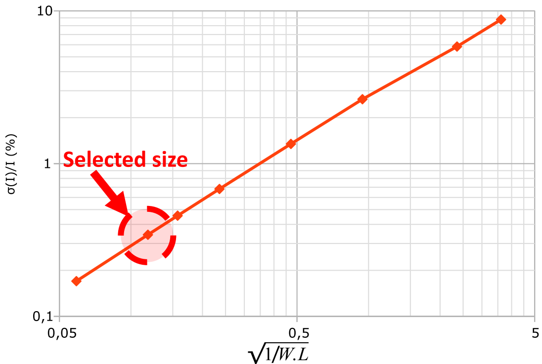
Figure 4.30: Technology matching for NMOS current mirror.
