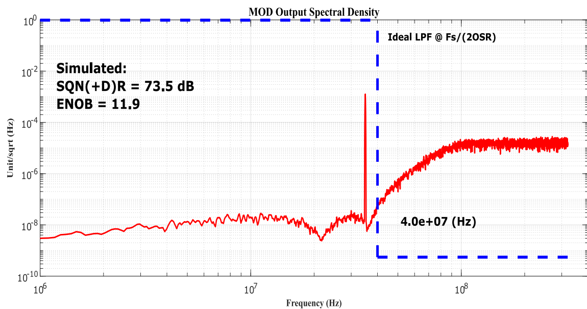
Figure 3.16: PSD of the proposed architecture with a sinwave input.
