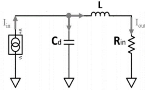
Figure 1.14: Precise equivalent electrical model of the input stage circuit with bonding wire inductance L .
