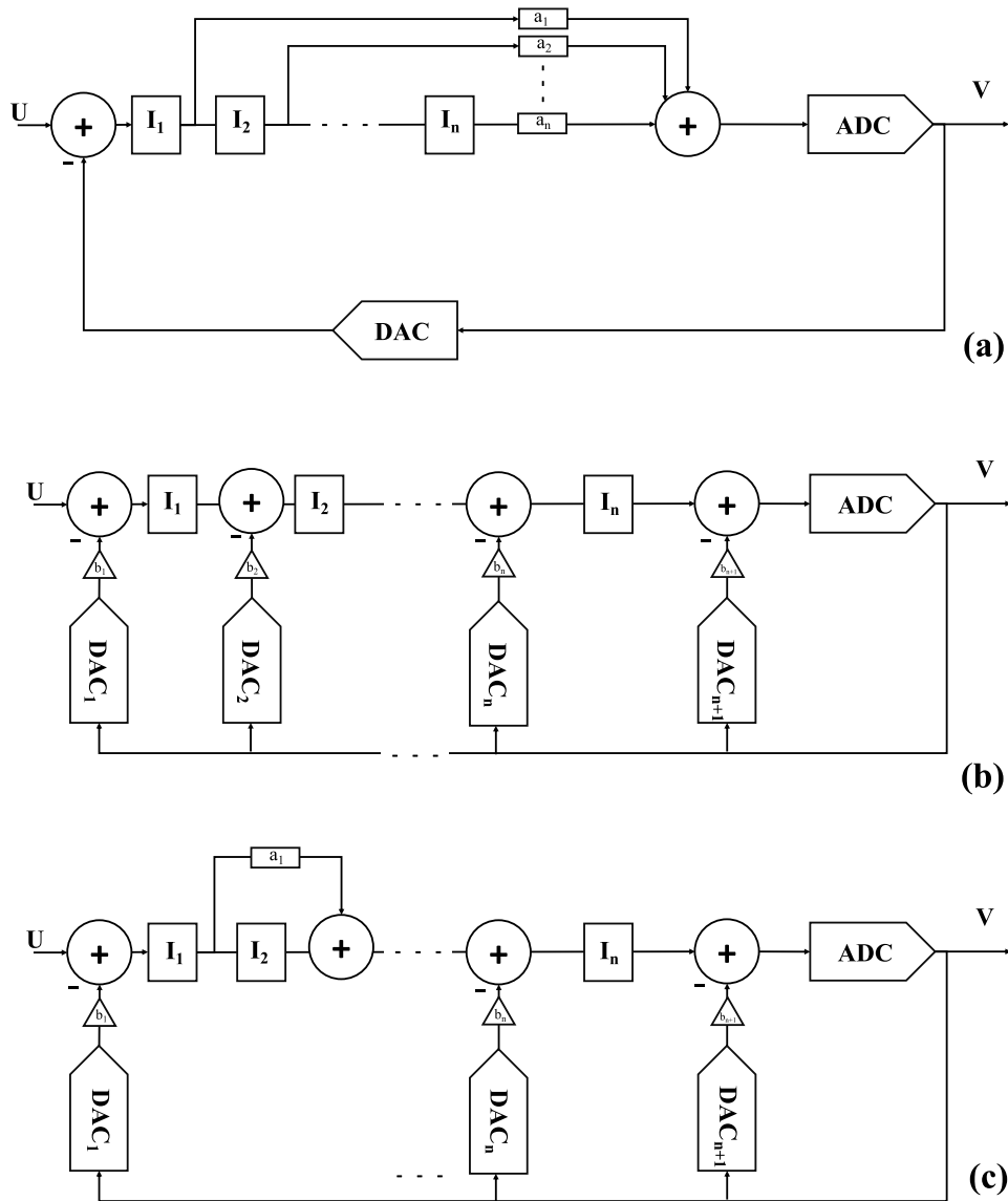
Figure 2.23: Different styles of compensation: (a): Feedforward loop filter; (b): Feedback loop filter; (c): Mixed feedforward-feedback loop filter.
