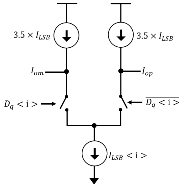
Figure 4.29: Simplified diagram of a differential current-steering DAC cell.
