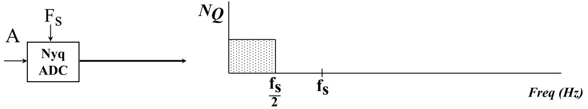
Figure 2.15: Power spectral density of quantization noise in Nyquist-rate ADC.
