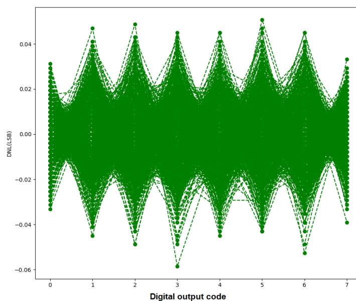
Figure 3.23: Extracted DNL values for a 3\text{ mV} ADC voltage error.
