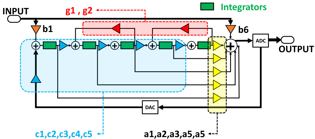
Figure 3.1: A simplified block diagram of the proposed CT \Delta\Sigma modulator.
