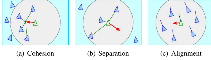
Figure 3.2.: Flocking rules known as steering behaviors applied to a simple Boids as represented by Reynolds. The rules known as cohesion, separation, and alignment are applied to each boi individually. The boi has full knowledge of the velocity, position, and heading of its neighbors in a certain range in order to compute its velocity and heading.
