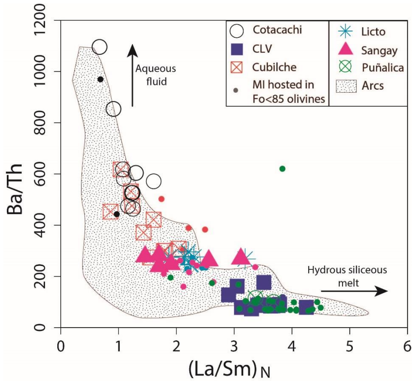
Figure 9 (\text{La}/\text{Sm})_N vs. \text{Ba}/\text{Th} for Ecuadorian MI. The arc basalt field is from Elliot (2003). Sangay MI shown with pink triangles and Puñalica MI compositions from Narváez et al. (2018). Th compositions are not available for PDA and Rucu Pichincha MI.
