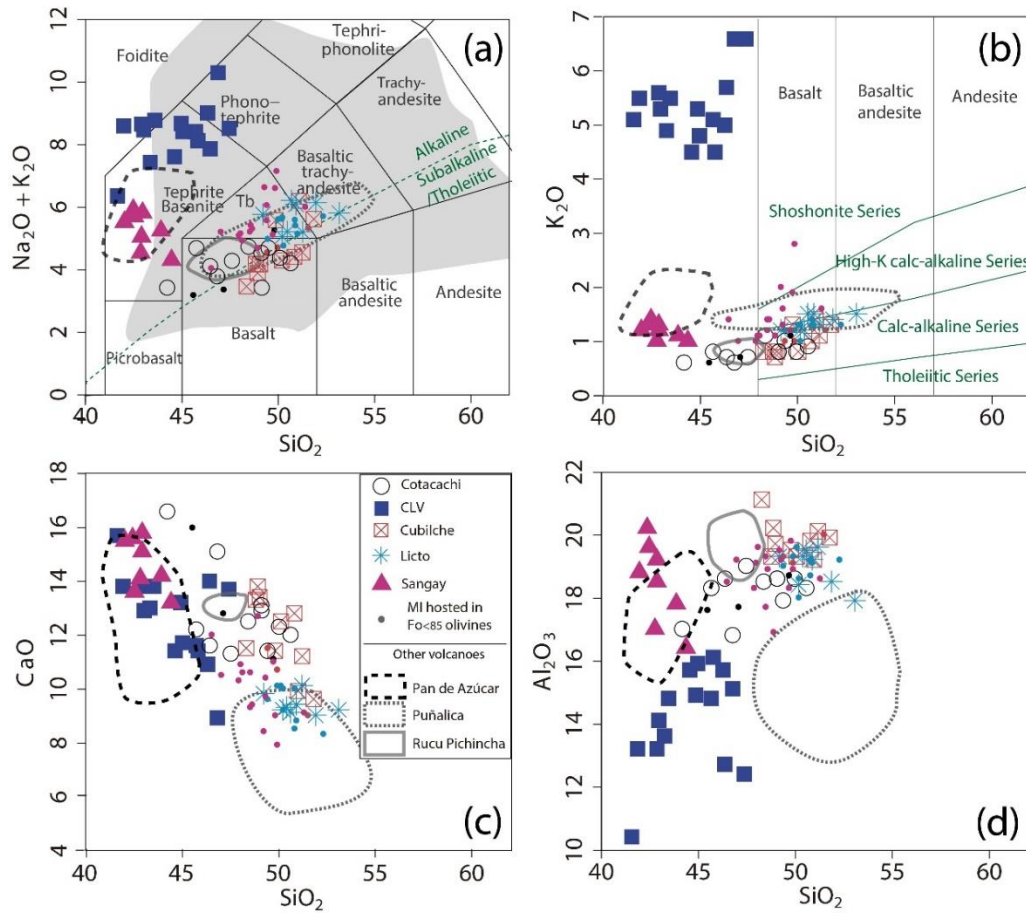
Figure 2 (a) SiO 2 vs. Na 2 O + K 2 O classification diagram (Le Bas et al., 1986) of olivine-hosted MI compositions from the Ecuadorian arc. MI are divided in two groups. MI hosted in Fo > 85 olivines are shown with larger colored symbols, while those hosted in Fo < 85 olivines are depicted with small colored filled circles to show potential compositional variations related to magma evolution. The colors are the same as the volcano color codes in Fig. 1. Sangay MI shown with pink triangles and Puñalica MI compositions from Narváez et al. (2018), PDA, and Rucu Pichincha MI from Le Voyer et al. (2008). The area labeled “Tb” corresponds to trachy-basalt field. The gray shade without a black border is the entire compositional variation of Ecuadorian quaternary volcanoes rocks (database from Ancellin et al., 2017). (b) SiO 2 vs. K 2 O classification diagram from Peccerillo and Taylor (1976). (c-d) Harker diagram of silica versus CaO and Al 2 O 3 wt.%. Plotted data are uncorrected for post-entrapment modifications, and are normalized for an anhydrous basis.
