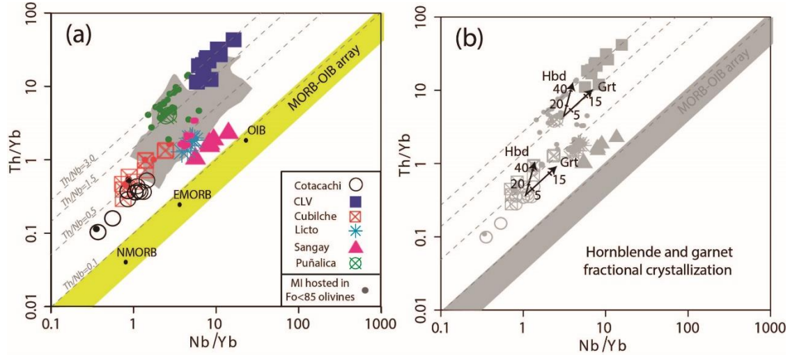
Figure 7 (a-b) Nb/Yb vs. Th/Yb of Ecuatorian MI compared to MORB-OIB compositions used to discriminate between conservative and non-conservative elements (Pearce et al., 2008). Th compositions are not available for PDA and Rucu Pichincha MI. The gray shade in (a) is the entire compositional variation of Ecuatorian quaternary volcanic rocks (data from Ancellin et al., 2017). The black arrow in (b) is the result of 45 and 20% fractional crystallization of a mono-mineral cumulate composed of hornblende and garnet, respectively, using D^{\text{mineral/melt}} for individual minerals in contact with basaltic melts given by Green et al. (2000). The corresponding arrows for other typical minerals (plagioclase, pyroxenes) are smaller than the size of the symbols. Sangay MI shown with pink triangles and Puñalica MI compositions from Narváez et al. (2018). Th compositions are not available for PDA and Rucu Pichincha MI.
