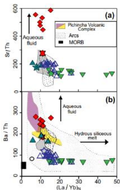
Fig. 8 Plot of (\text{La/Yb})_N normalized to primitive mantle (Sun and McDonough 1989) vs. a Sr/Th and b Ba/Th. Whole-rock data variation for Pichincha Volcanic Complex field is taken from Samaniego et al. (2010). Purple field corresponds to the older Rucu Pichincha magmatic suite, whereas yellow field corresponds the younger Guagua Pichincha suite. MORB composition represented by the small black rectangle is from Leroux et al. (2006). The primitive arc magma composition (dotted field) is taken from Elliott (2003). Symbols are those of Fig. 2
