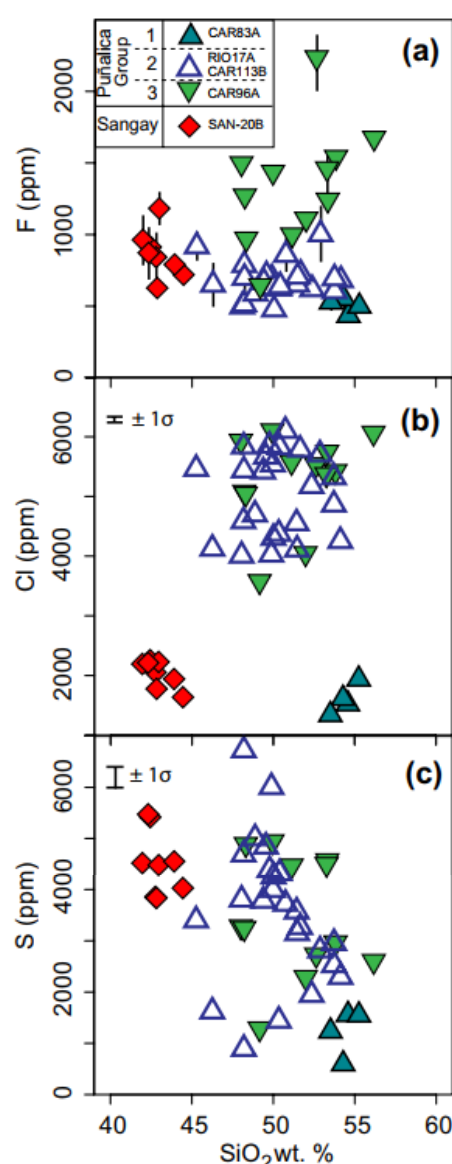
Fig. 5 F, Cl, and S vs. \text{SiO}_2 of Puñalica and Sangay melt inclusions. Standard error of the mean values ( \pm 1\sigma ) are shown as vertical lines
