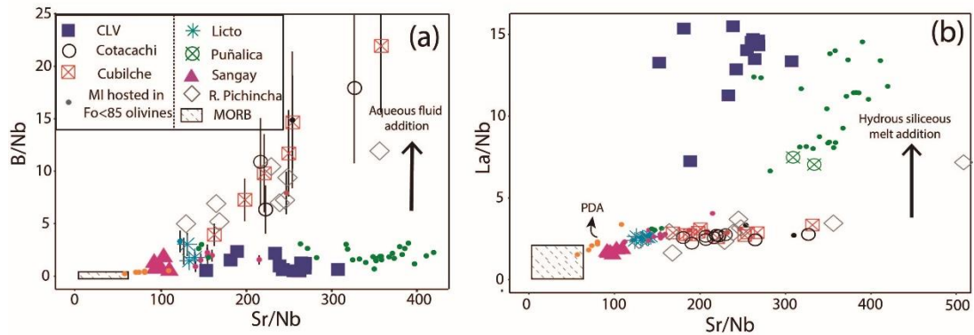
Figure 8 (a) \text{Sr/Nb} vs. \text{B/Nb} and (b) \text{Sr/Nb} vs. \text{La/Nb} for Ecuadorian MI. Propagated standard error bars ( \pm 1\sigma ) of new data are shown in vertical lines in (a). The hatched boxes in (a) and (b) are MORB fields based on data from Leroux et al. (2006) and Chaussidon and Marty (1995). Sangay MI shown with pink triangles and Puñalica MI compositions from Narváez et al. (2018), PDA, and Rucu Pichincha MI from Le Voyer et al. (2008).
