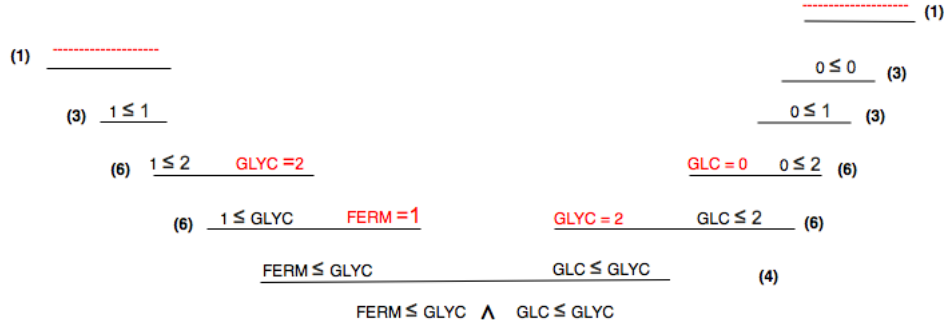
Figure 11.2: Proof tree proving \text{FERM} \leq \text{GLYC} using inference rules. Dotted lines and red text refer to the leaves of the proof tree.
