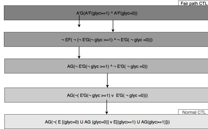
Figure 5.27: Standard CTL equivalent of fair path CTL of the variable x tending towards a specific threshold (here 2).
