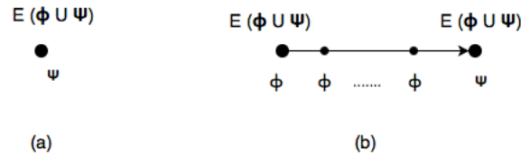
Figure 3.18: Model checking using E(\phi \cup \psi) . (a) A state where \psi holds can be labelled as E(\phi \cup \psi) (b) If the predecessor of this state satisfies \phi , then the predecessor can also be labelled E(\phi \cup \psi) .
