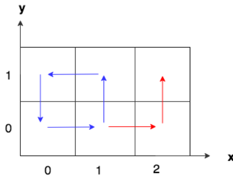
Figure 6.7: State transition graph showing the dynamics between x and y , when c=1 .
