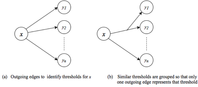
Figure 5.3: (a) Using outgoing edges to identify thresholds for each variable. (b) x \rightarrow y_1 and x \rightarrow y_2 have the same thresholds and therefore are grouped together.
