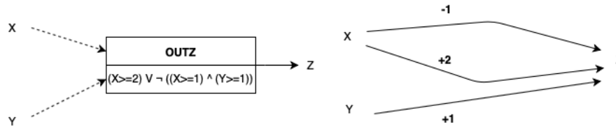
Figure 6.22: (Left) A multiplex where the variable X appears twice in the formula with different thresholds. In this example Z has only one possible resource (OUTZ), thus 2 parameters K_Z, \dots (Right) Its translation into a Thomas network without multiplexes. Z has then 3 possible resources, thus 8 parameters, and the respective values of the parameters have to reflect the truth table of the formula of the original multiplex.
