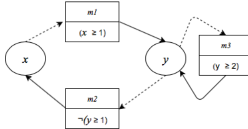
Figure 4.10: An interaction graph with multiplexes as resources. \neg means inhibition. Doted lines are only drawn to facilitate the global view: They can be deduced from the multiplex formulas.
