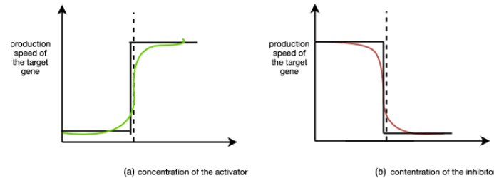
Figure 4.1: Discretisation of sigmoids (a) Activation (b) Inhibition
