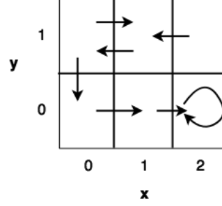
Figure 3.14: Example of a state transition graph: stable state ( x=2,y=0 ), its attraction basin (covering states starting from x=0,y=0 ) and infinite loop (transitions between states 1,1 and 0,1)
