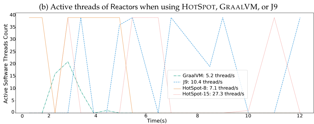
Figure 5.6: Active threads evolution when using HOTSPOT, GRAALVM, or J9
