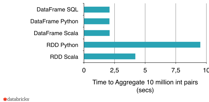
Fig. 7.4.: Benchmark of an aggregation task in Spark with RDD and DataFrame APIs in different languages.
