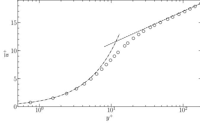
Figure 1.4: Mean velocity profile of an equilibrium turbulent boundary layer at \text{Re}_\tau = u_\tau \delta / \nu = 395 . \circ , DNS profile from Appendix A; \cdots , linear law u^+ = y^+ ; --- logarithmic law u^+ = (1/0.4) \ln y^+ + 5.5 .
