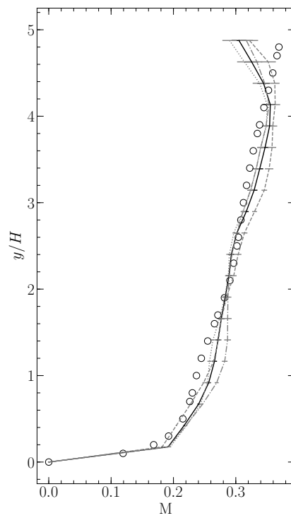
Figure 6.8: Validation of the test-rig. Comparison of specified Mach profile with values obtained in the experiments at UMS1. \circ , specified profile of Section 6.3; — experimental profile averaged along z^H \in [-1, 1] ; \cdots exp. profile at z^H = 0 ; -\cdot- exp. profile at z^H = 1 ; - - - exp. profile at z^H = -1 .
