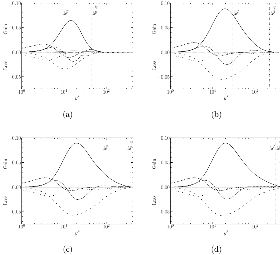
Figure 3.21: Budgets of wall-normal turbulent heat flux at x/\delta = 0.73 (a), 2\pi (b), 5.7\pi (c) and 16.5\pi : — streamwise ( VI_x : gray) and wall-normal ( VI_y : black) production; - - - - - molecular dissipation III ; - - - - - streamwise ( II_x : gray) and wall-normal ( II_y : black) molecular diffusion; - · - · - streamwise ( VII_x : gray) and wall-normal ( VII_y : black) turbulent diffusion; · · · · · streamwise ( I_x : gray) and wall-normal ( I_y : black) convective terms; - - - - - enthalpy-pressure-gradient correlation IV .
