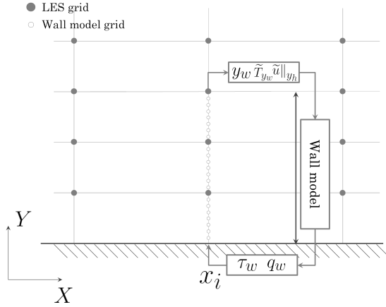
Figure 1.6: Schematic representation of the functioning of the TBLE equilibrium wall-model.
