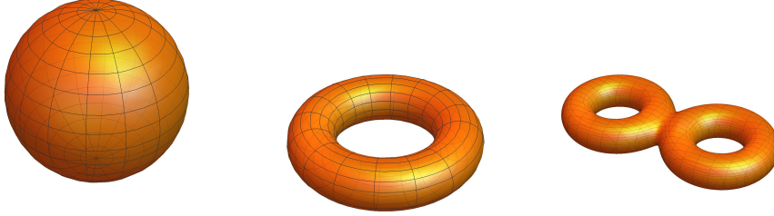
FIGURE 1.1: Topological manifolds with different genera g . Left: A sphere with g = 0 . Middle: A torus with g = 1 . Right: A double-torus with g = 2 .
