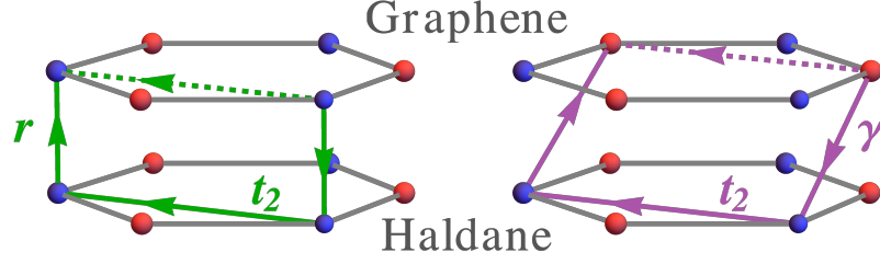
FIGURE 3.1: Schematic of the system and of the coupling parameters between the two systems. Left: Interlayer hopping between the same sublattice sites with hopping amplitude r . Right: Inter-layer hopping between neighboring sublattice sites with hopping amplitude \gamma .
