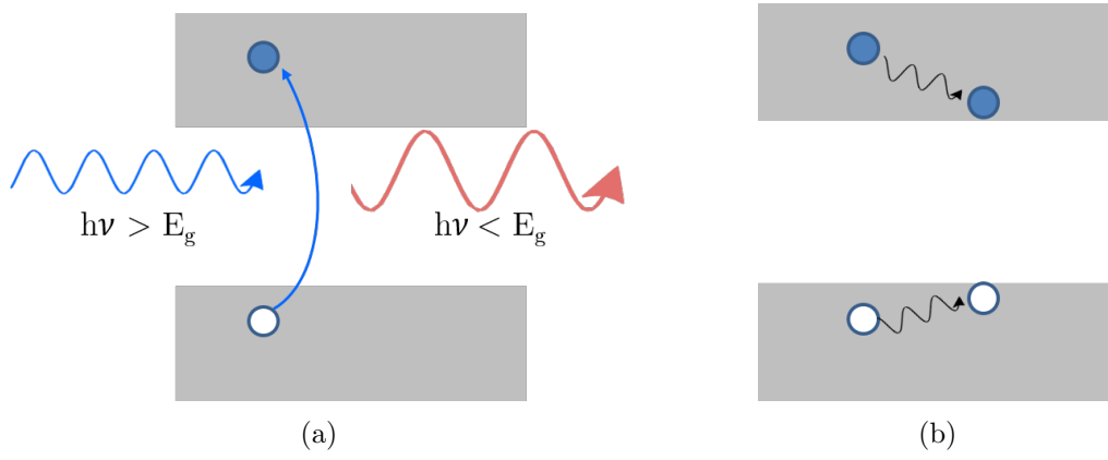
Figure 1.5: (a) Schematic of incomplete absorption of the solar spectrum: the red photon (energy lower than band-gap) is not absorbed, while the blue photon is (energy larger than the band-gap). (b) Thermalization loss of the excited electron and hole.
