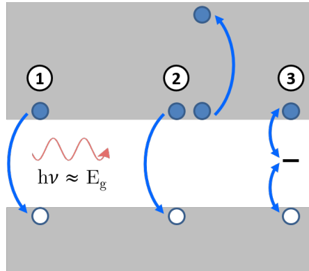
Figure 1.7: Schematic representation of recombination mechanisms: ① radiative, ② Auger, and ③ SRH recombinations.
