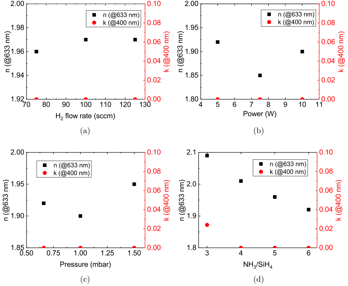
Figure 2.29: Evolution of n and k with (a) H 2 flow rate, (b) RF Power, (c) Pressure, and (d) NH 3 /SiH 4 flow rate ratio for the a-Si x N y H z deposition.
