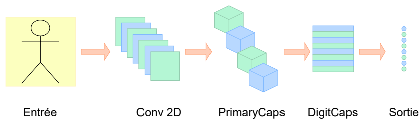
FIGURE 2.11 – Exemple d'architecture capsule network - partie classification
