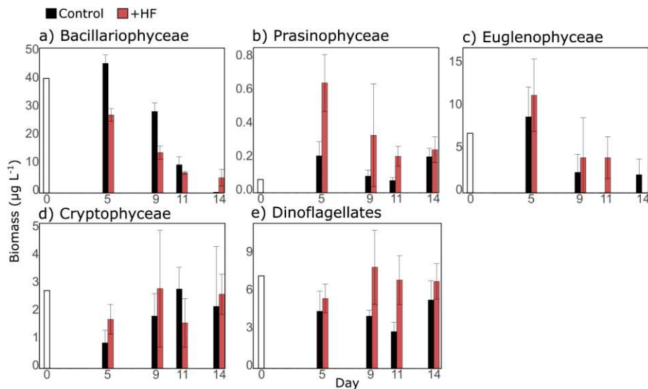
Figure 5. Mean biomass ( \mu\text{g L}^{-1} ) for major phytoplankton taxa with standard deviations (error bars) during five days of the experiment (d 0, d 5, d 9, d 11, and d 14) in the control (black) and +HF (red) treatments. The sample on d 0 was taken directly into the bay few minutes before filling the mesocosms and is represented in white. Note that the scales of the y-axes are different. a) Bacillariophyceae; b) Prasinophyceae; c) Euglenophyceae; d) Cryptophyceae; e) Dinoflagellates.
