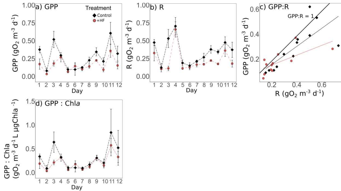
Figure 2. (a) Mean gross primary production (GPP) and (b) mean community respiration (R) with standard deviations (error bars) over time in the control (black diamonds) and the +HF treatment (red circles); (c) gross primary production (GPP): respiration (R) ratio in the control (black diamonds) and the +HF treatment (red circles). GPP: R > 1 indicates an autotrophic system, while GPP: R < 1 indicates a heterotrophic system; (d) Mean photosynthetic efficiency (expressed as GPP : Chlorophyll- a ratio) with standard deviations (error bars) over time in the control (black diamonds) and the +HF treatment (red circles).
