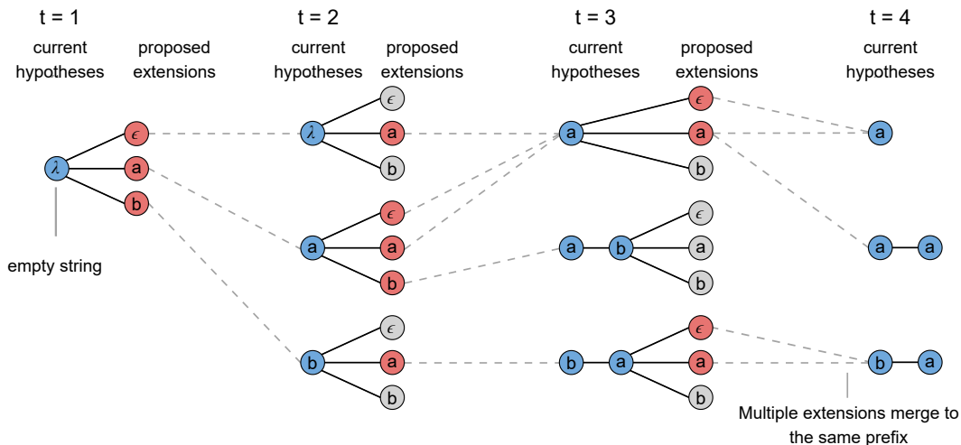
Figure 3.9 – A prefix CTC beam search algorithm with an alphabet of \{\epsilon, a, b\} and a beam size of three. In this case, the top three prefixes are kept at each time step t . The probability of one prefix is obtained by summing probabilities of all alignments mapping to it. This figure is reproduced from [Han17]. It is licensed under Creative Commons Attribution 4.0 Int. Permission is granted for reuse.
