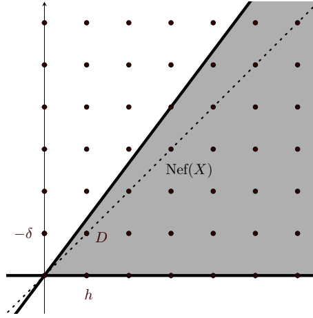
Figure 4.3.1: The nef cone of S_4^{[2]}
