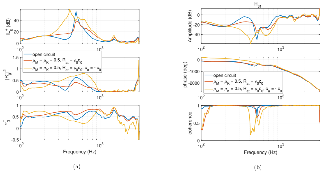
Figure 3.43: Comparison among the open circuit, the local and advection control laws in terms of scattering performances (a) and the transfer function H_{31} (b).
